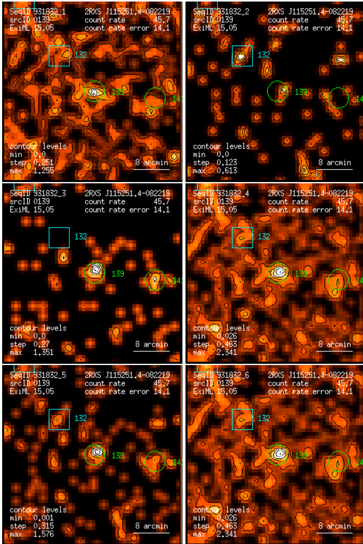
Figure 139: RASS 931832: detection 0139: band rate images, Gaussian filter: (1) PSPC channels 11 – 41, (2) 52 – 90, (3) 91 – 201, (4) 11 – 235, (5) 52 – 201, (6) 11 – 201. Broad band rates in counts/ks. Band rate contour levels in counts/ks/arcmin 2 .
