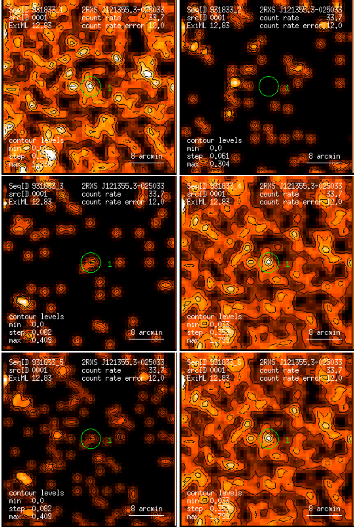
Figure 1: RASS 931833: detection 0001: band rate images, Gaussian filter: (1) PSPC channels 11 – 41, (2) 52 – 90, (3) 91 – 201, (4) 11 – 235, (5) 52 – 201, (6) 11 – 201. Broad band rates in counts/ks. Band rate contour levels in counts/ks/arcmin 2 .
