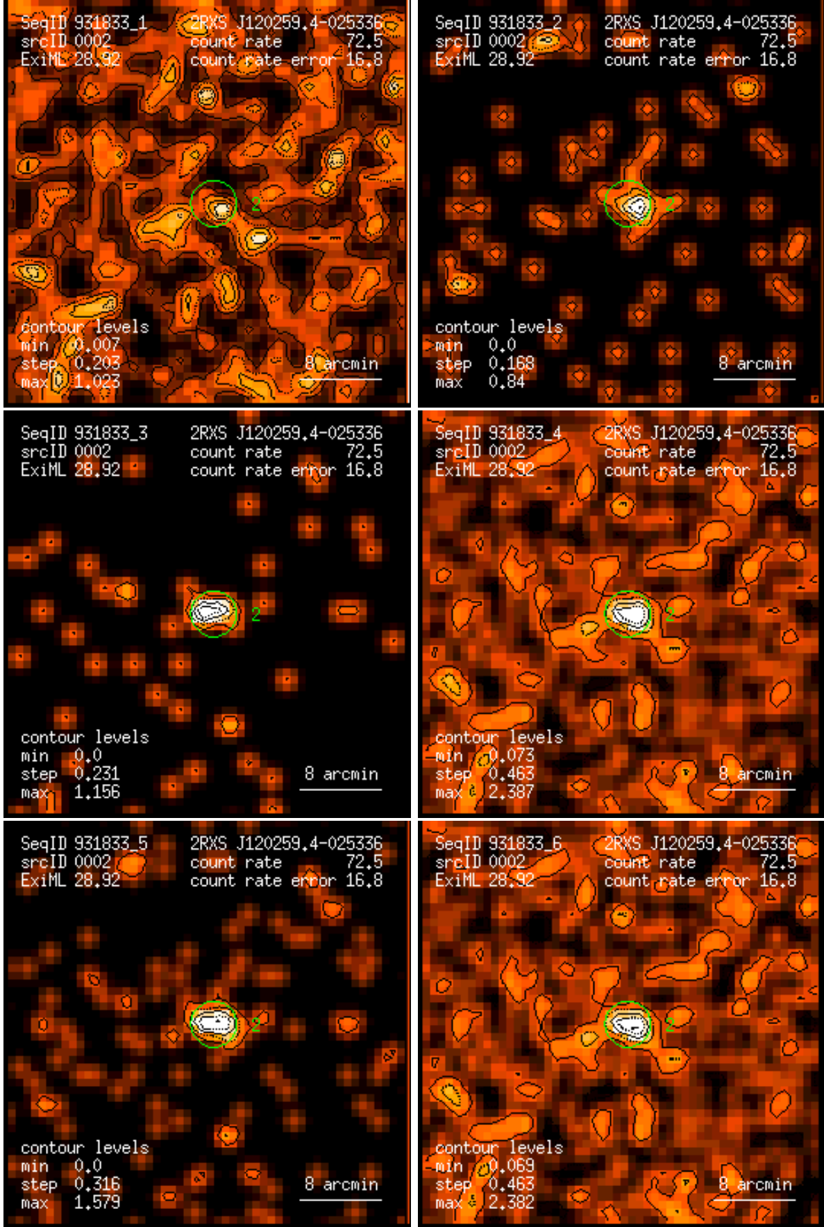
Figure 2: RASS 931833: detection 0002: band rate images, Gaussian filter: (1) PSPC channels 11 – 41, (2) 52 – 90, (3) 91 – 201, (4) 11 – 235, (5) 52 – 201, (6) 11 – 201. Broad band rates in counts/ks. Band rate contour levels in counts/ks/arcmin 2 .
