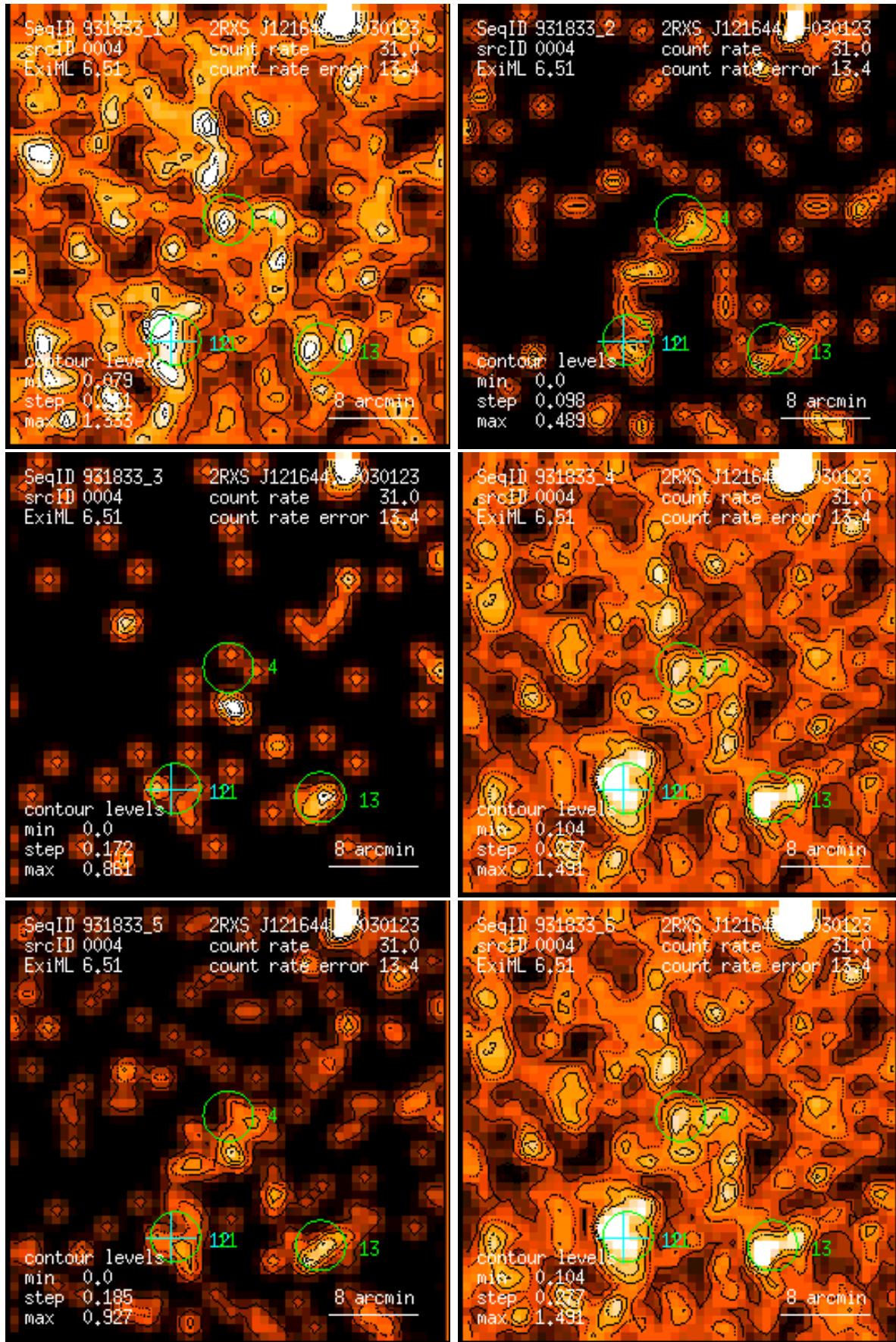
Figure 4: RASS 931833: detection 0004: band rate images, Gaussian filter: (1) PSPC channels 11 – 41, (2) 52 – 90, (3) 91 – 201, (4) 11 – 235, (5) 52 – 201, (6) 11 – 201. Broad band rates in counts/ks. Band rate contour levels in counts/ks/arcmin 2 .
