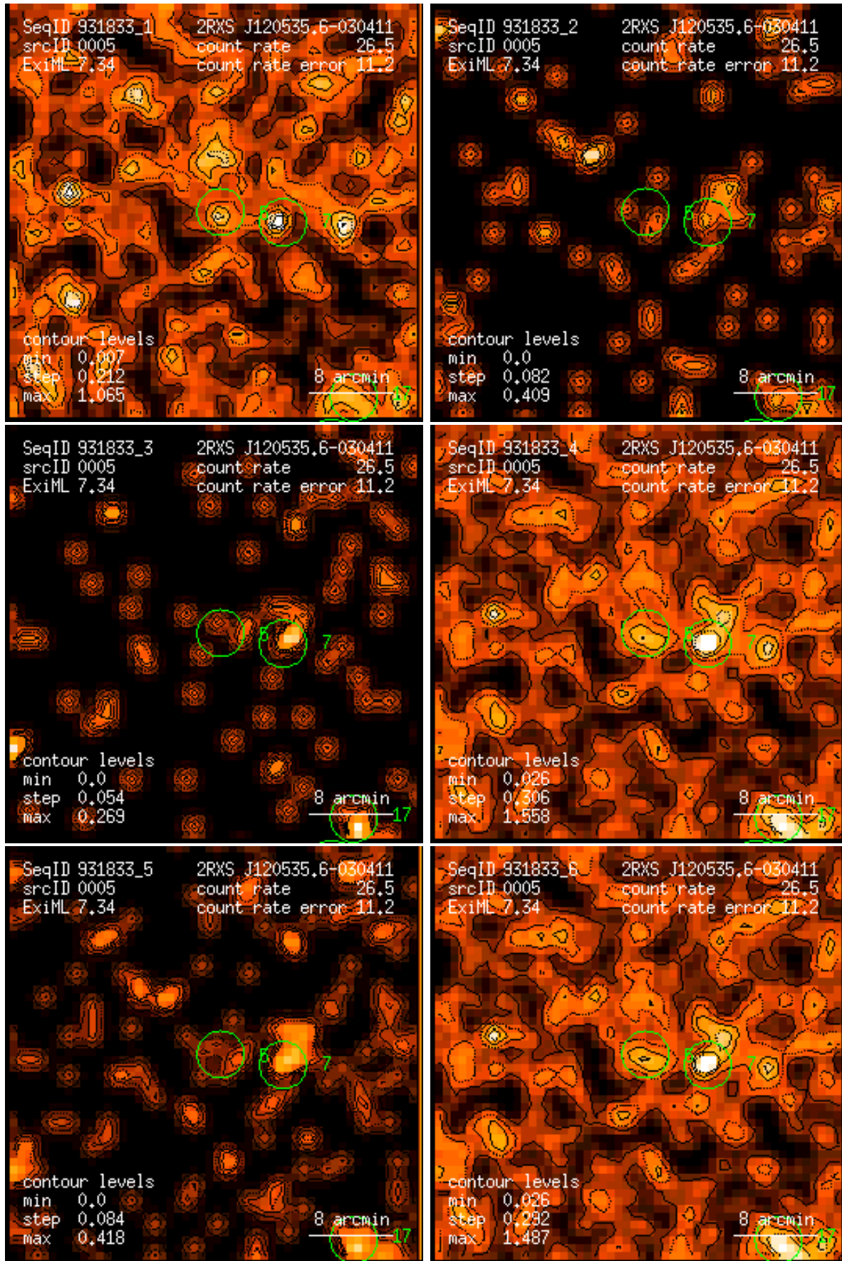
Figure 5: RASS 931833: detection 0005: band rate images, Gaussian filter: (1) PSPC channels 11 – 41, (2) 52 – 90, (3) 91 – 201, (4) 11 – 235, (5) 52 – 201, (6) 11 – 201. Broad band rates in counts/ks. Band rate contour levels in counts/ks/arcmin 2 .
