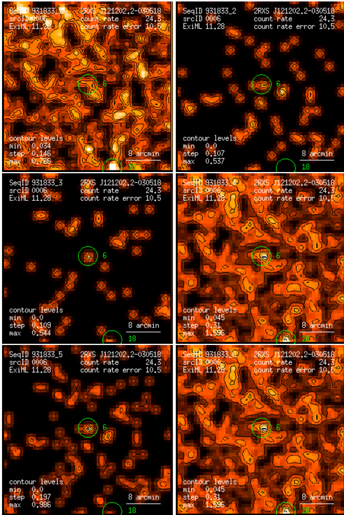
Figure 6: RASS 931833: detection 0006: band rate images, Gaussian filter: (1) PSPC channels 11 – 41, (2) 52 – 90, (3) 91 – 201, (4) 11 – 235, (5) 52 – 201, (6) 11 – 201. Broad band rates in counts/ks. Band rate contour levels in counts/ks/arcmin 2 .
