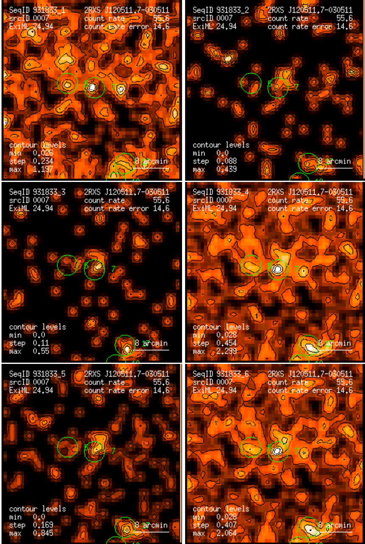
Figure 7: RASS 931833: detection 0007: band rate images, Gaussian filter: (1) PSPC channels 11 – 41, (2) 52 – 90, (3) 91 – 201, (4) 11 – 235, (5) 52 – 201, (6) 11 – 201. Broad band rates in counts/ks. Band rate contour levels in counts/ks/arcmin 2 .
