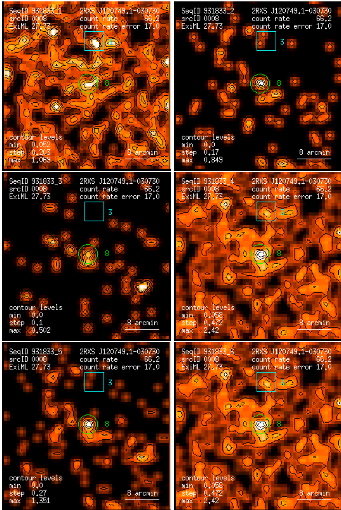
Figure 8: RASS 931833: detection 0008: band rate images, Gaussian filter: (1) PSPC channels 11 – 41, (2) 52 – 90, (3) 91 – 201, (4) 11 – 235, (5) 52 – 201, (6) 11 – 201. Broad band rates in counts/ks. Band rate contour levels in counts/ks/arcmin 2 .
