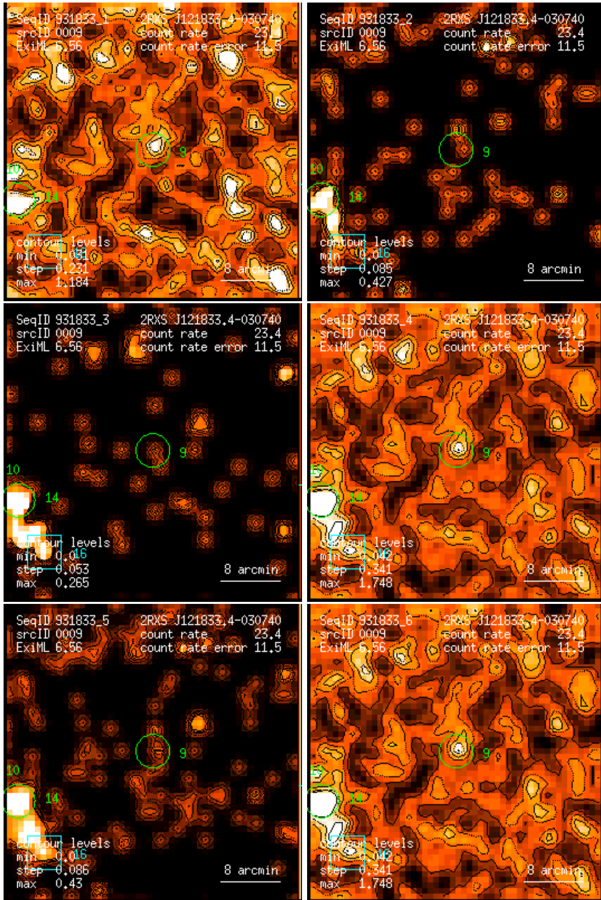
Figure 9: RASS 931833: detection 0009: band rate images, Gaussian filter: (1) PSPC channels 11 – 41, (2) 52 – 90, (3) 91 – 201, (4) 11 – 235, (5) 52 – 201, (6) 11 – 201. Broad band rates in counts/ks. Band rate contour levels in counts/ks/arcmin 2 .
