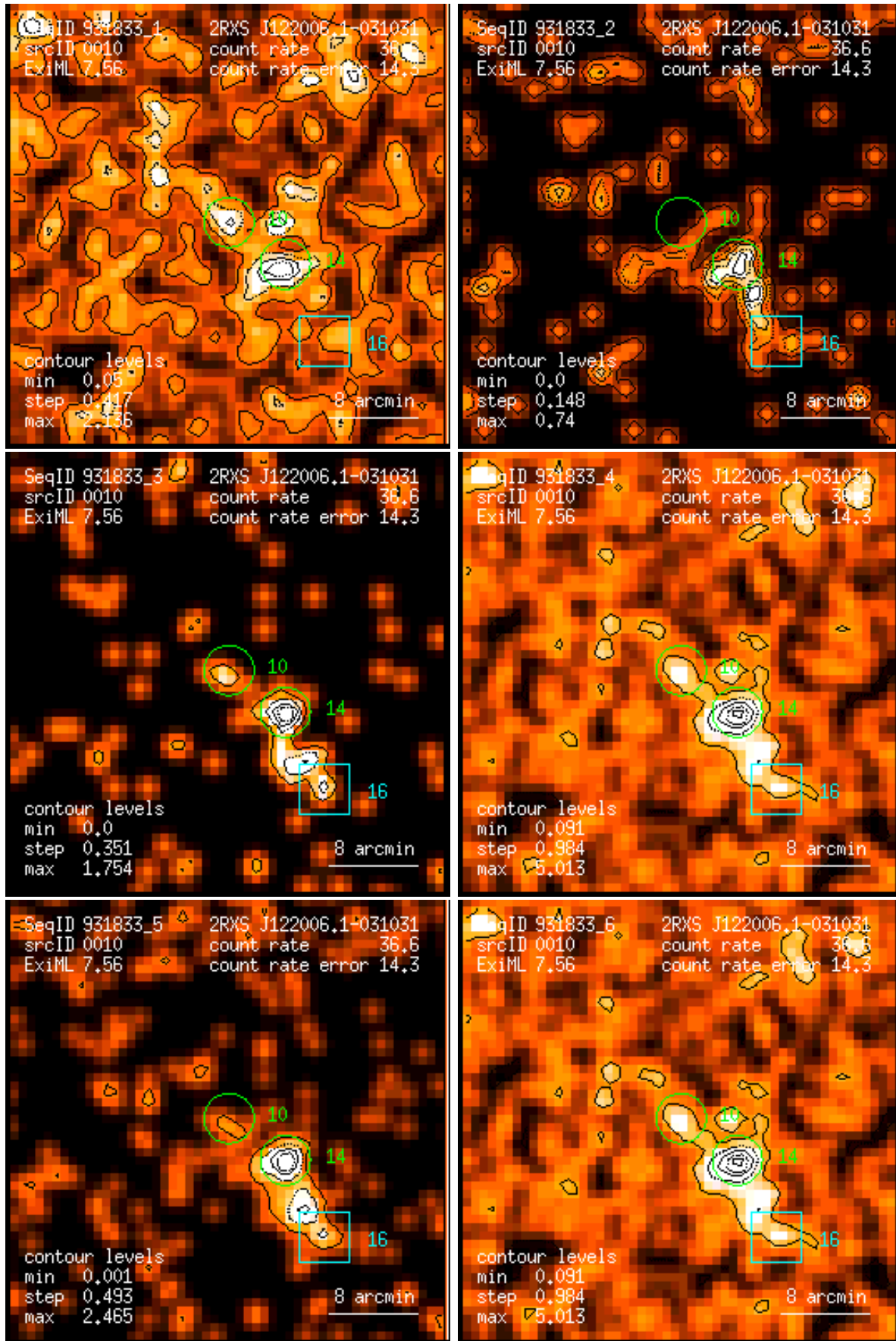
Figure 10: RASS 931833: detection 0010: band rate images, Gaussian filter: (1) PSPC channels 11 – 41, (2) 52 – 90, (3) 91 – 201, (4) 11 – 235, (5) 52 – 201, (6) 11 – 201. Broad band rates in counts/ks. Band rate contour levels in counts/ks/arcmin 2 .
