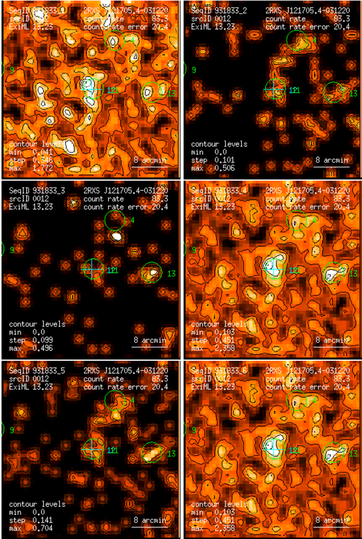
Figure 12: RASS 931833: detection 0012: band rate images, Gaussian filter: (1) PSPC channels 11 – 41, (2) 52 – 90, (3) 91 – 201, (4) 11 – 235, (5) 52 – 201, (6) 11 – 201. Broad band rates in counts/ks. Band rate contour levels in counts/ks/arcmin 2 .
