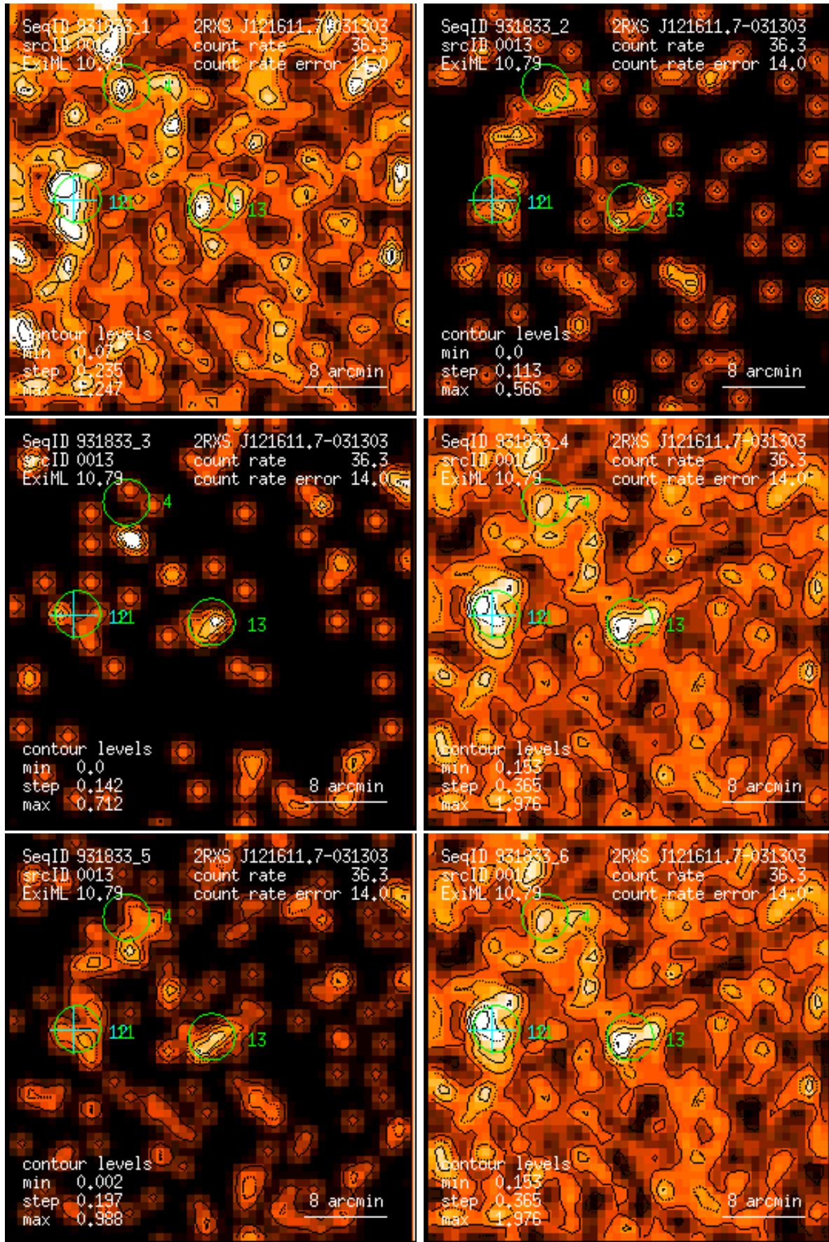
Figure 13: RASS 931833: detection 0013: band rate images, Gaussian filter: (1) PSPC channels 11 – 41, (2) 52 – 90, (3) 91 – 201, (4) 11 – 235, (5) 52 – 201, (6) 11 – 201. Broad band rates in counts/ks. Band rate contour levels in counts/ks/arcmin 2 .
