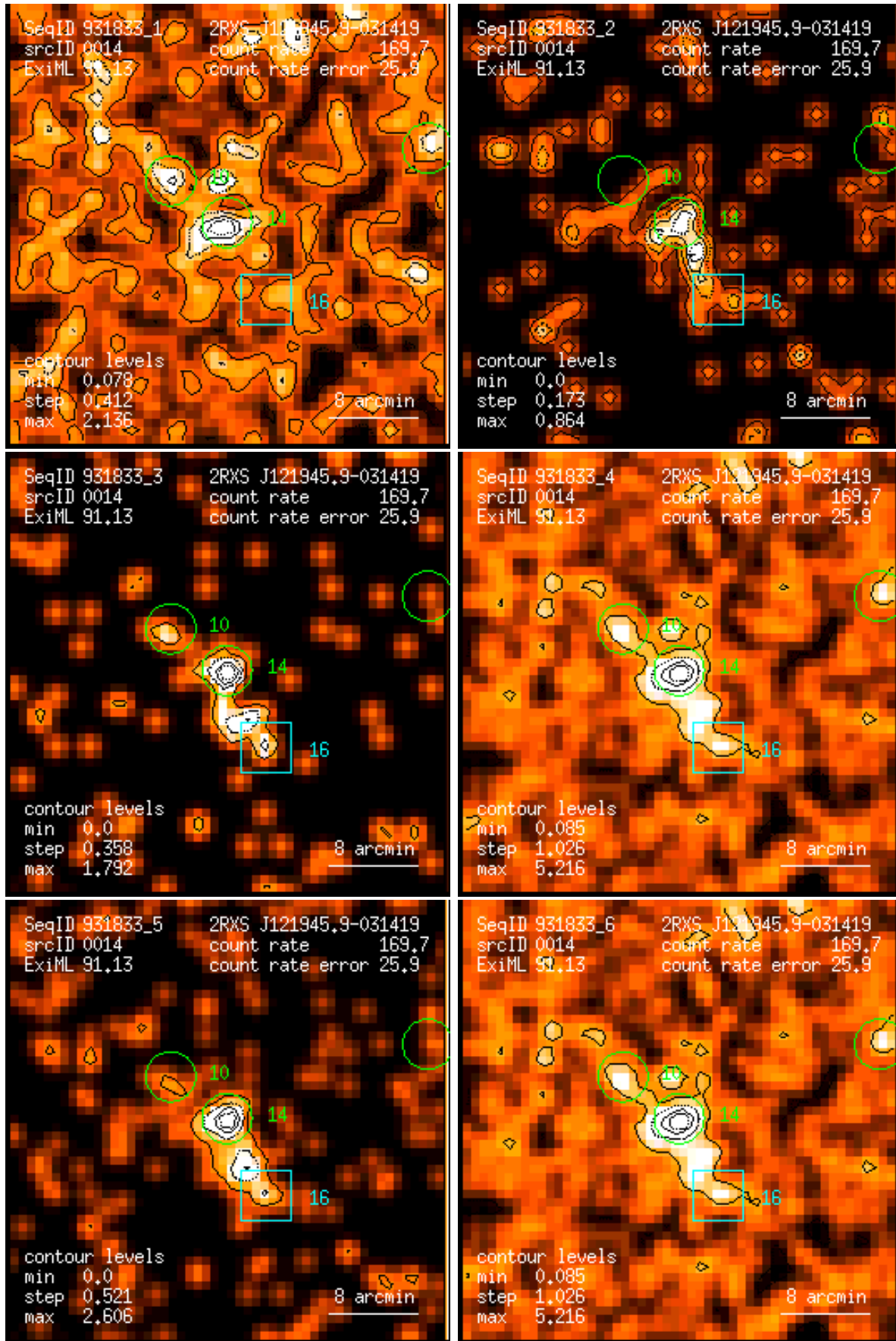
Figure 14: RASS 931833: detection 0014: band rate images, Gaussian filter: (1) PSPC channels 11 – 41, (2) 52 – 90, (3) 91 – 201, (4) 11 – 235, (5) 52 – 201, (6) 11 – 201. Broad band rates in counts/ks. Band rate contour levels in counts/ks/arcmin 2 .
