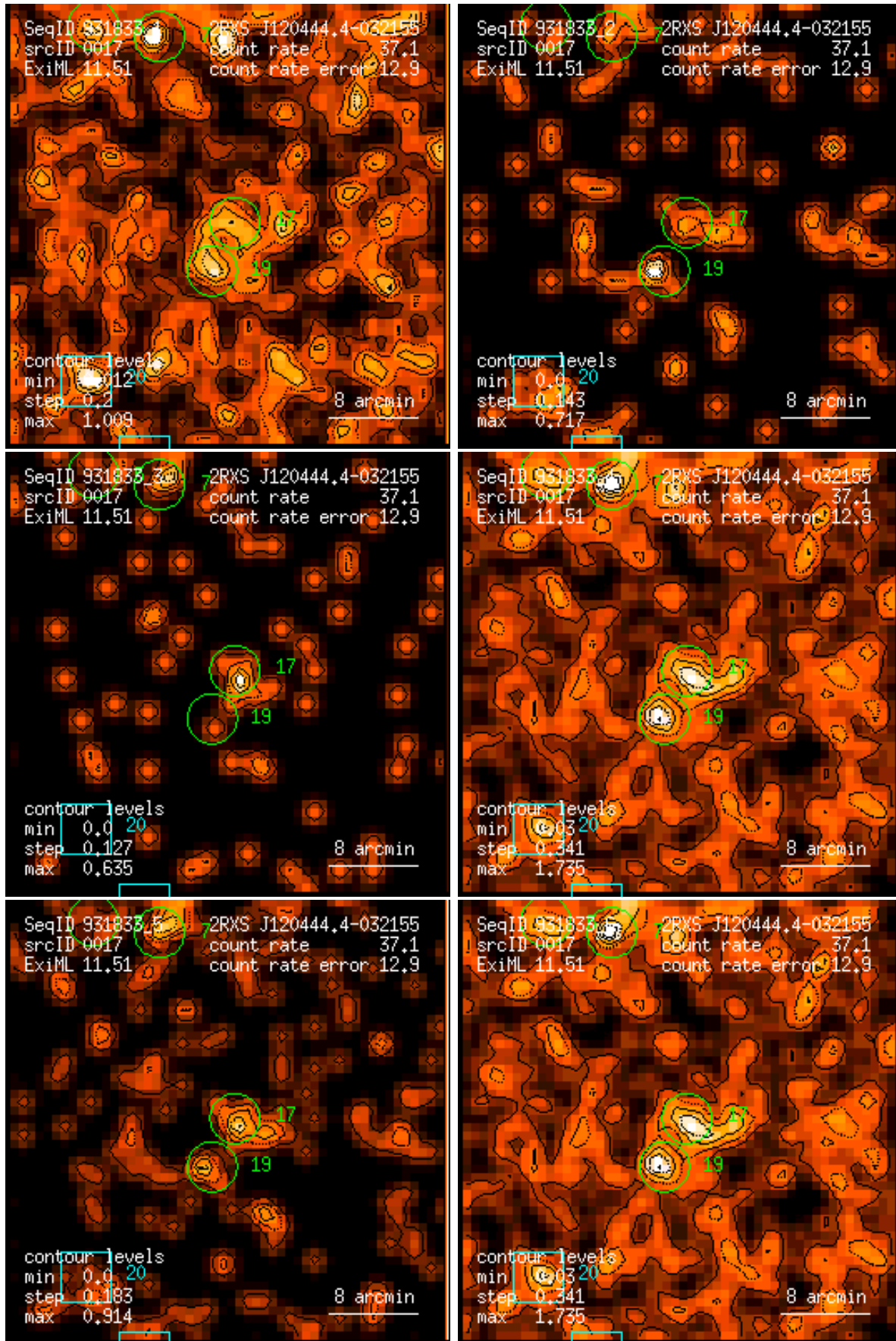
Figure 17: RASS 931833: detection 0017: band rate images, Gaussian filter: (1) PSPC channels 11 – 41, (2) 52 – 90, (3) 91 – 201, (4) 11 – 235, (5) 52 – 201, (6) 11 – 201. Broad band rates in counts/ks. Band rate contour levels in counts/ks/arcmin 2 .
