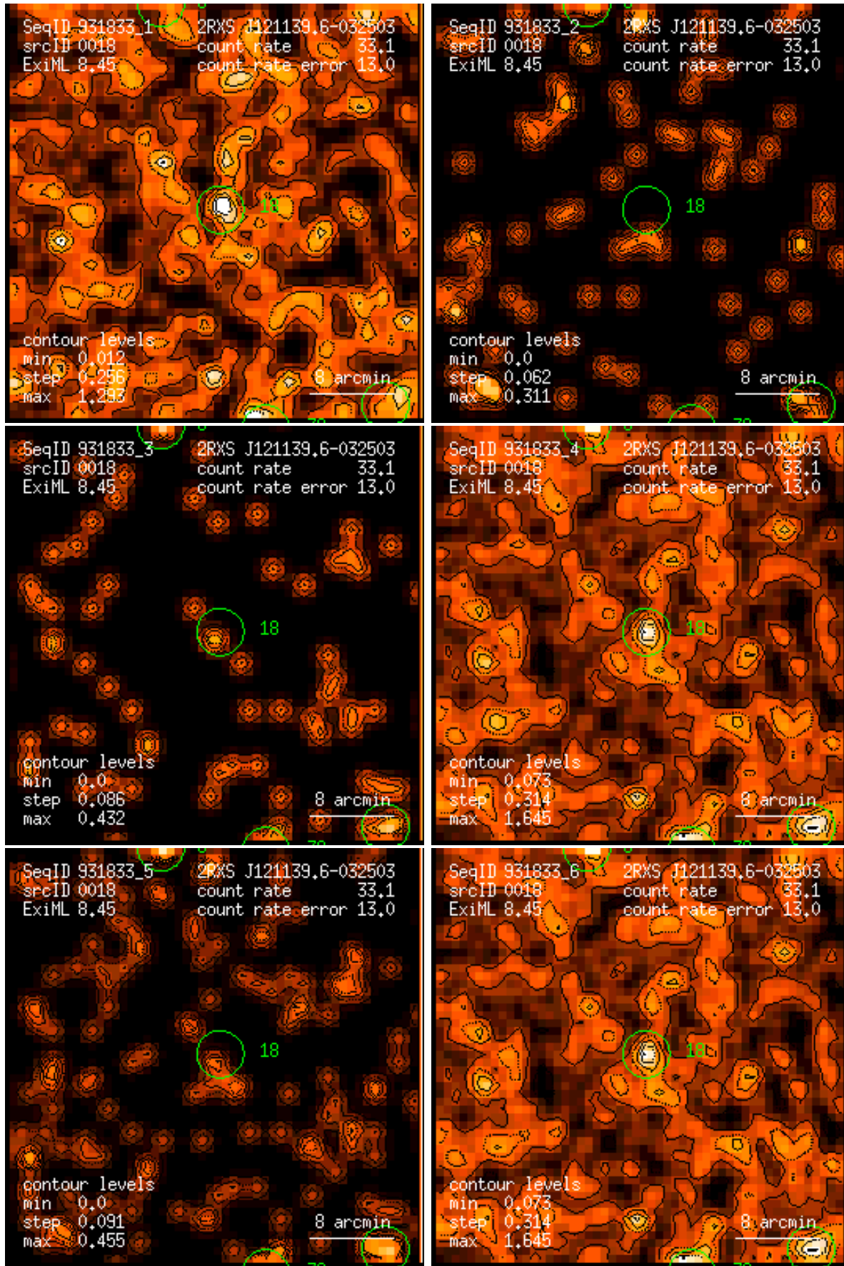
Figure 18: RASS 931833: detection 0018: band rate images, Gaussian filter: (1) PSPC channels 11 – 41, (2) 52 – 90, (3) 91 – 201, (4) 11 – 235, (5) 52 – 201, (6) 11 – 201. Broad band rates in counts/ks. Band rate contour levels in counts/ks/arcmin 2 .
