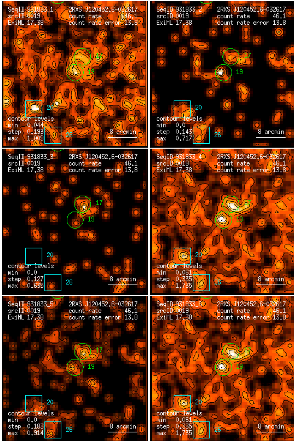
Figure 19: RASS 931833: detection 0019: band rate images, Gaussian filter: (1) PSPC channels 11 – 41, (2) 52 – 90, (3) 91 – 201, (4) 11 – 235, (5) 52 – 201, (6) 11 – 201. Broad band rates in counts/ks. Band rate contour levels in counts/ks/arcmin 2 .
