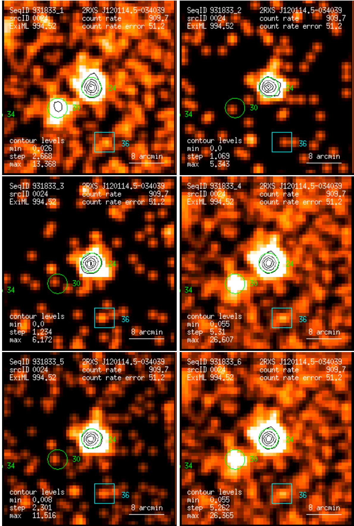
Figure 24: RASS 931833: detection 0024: band rate images, Gaussian filter: (1) PSPC channels 11 – 41, (2) 52 – 90, (3) 91 – 201, (4) 11 – 235, (5) 52 – 201, (6) 11 – 201. Broad band rates in counts/ks. Band rate contour levels in counts/ks/arcmin 2 .
