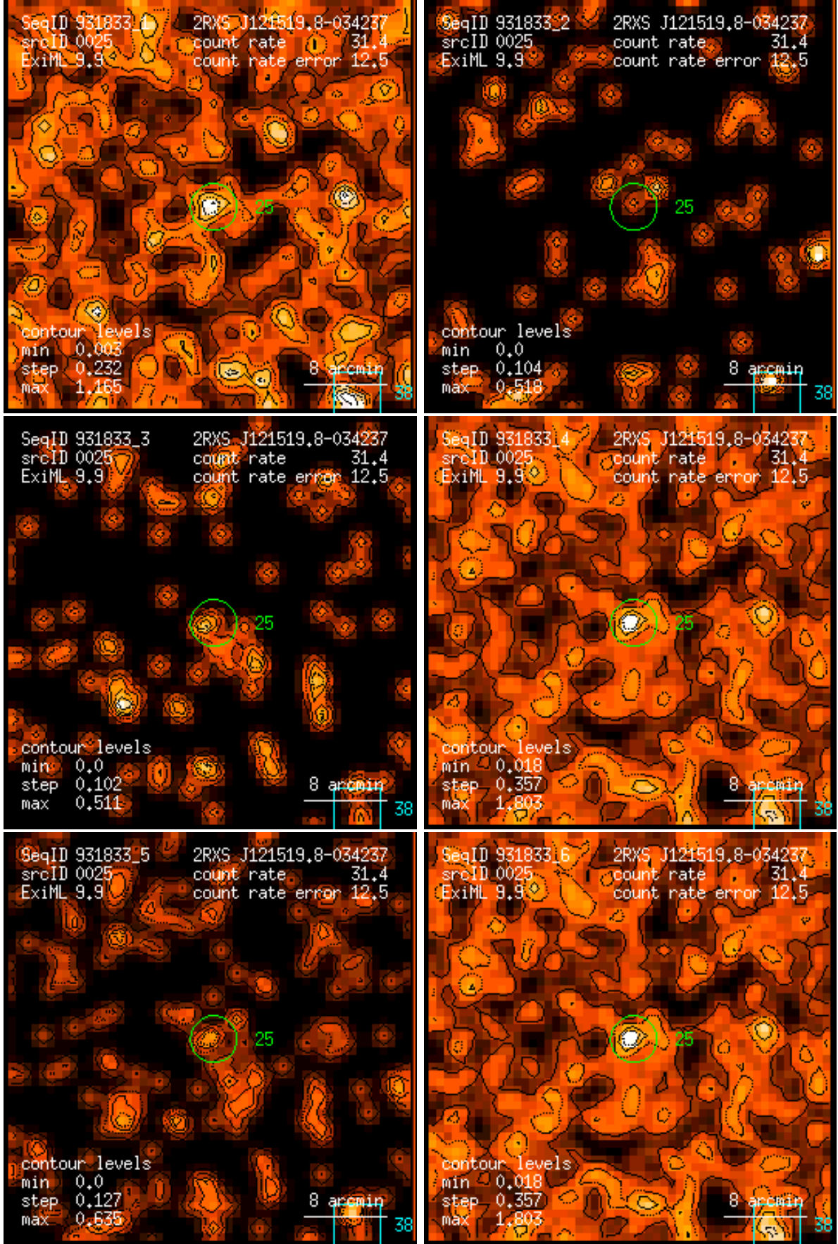
Figure 25: RASS 931833: detection 0025: band rate images, Gaussian filter: (1) PSPC channels 11 – 41, (2) 52 – 90, (3) 91 – 201, (4) 11 – 235, (5) 52 – 201, (6) 11 – 201. Broad band rates in counts/ks. Band rate contour levels in counts/ks/arcmin 2 .
