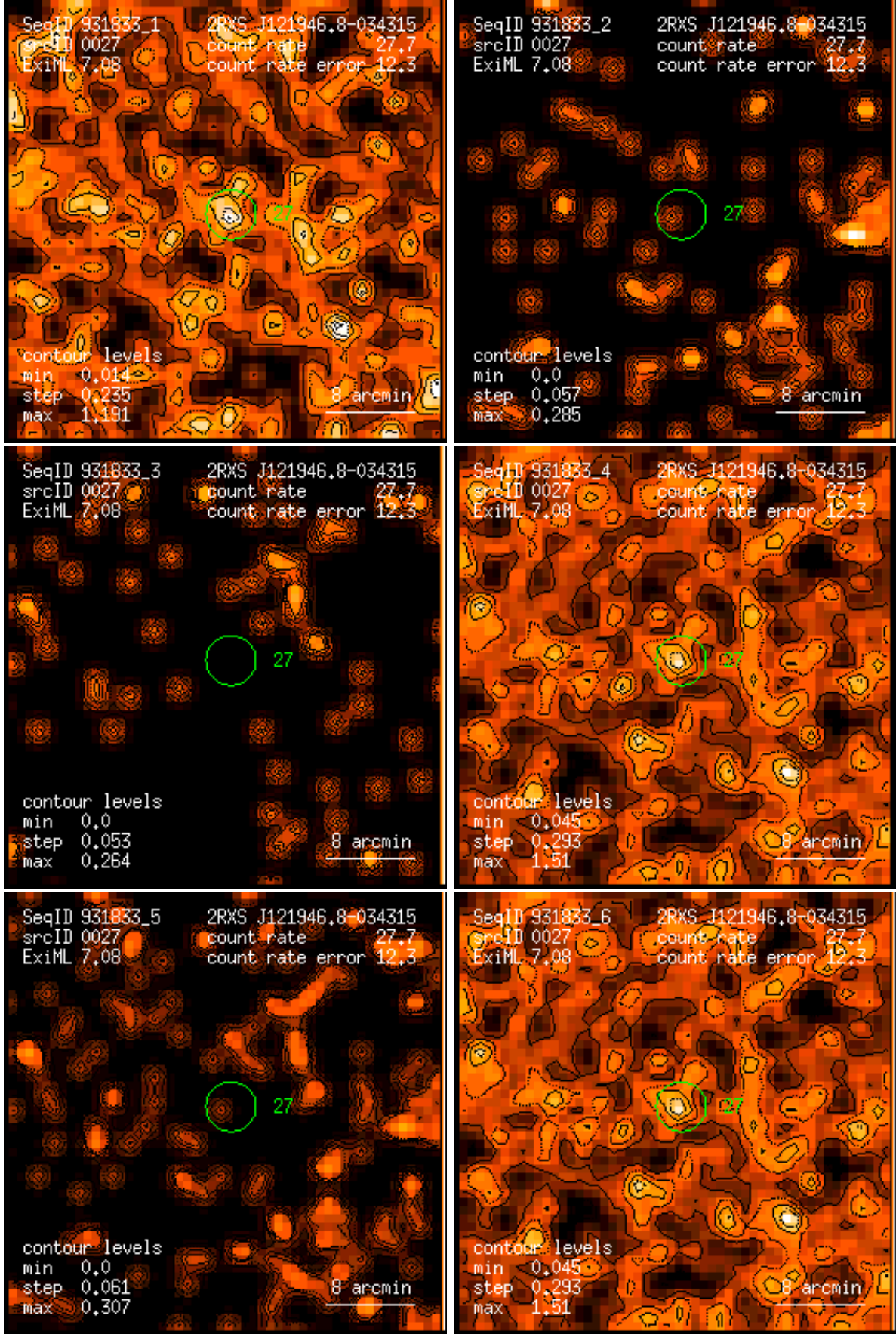
Figure 27: RASS 931833: detection 0027: band rate images, Gaussian filter: (1) PSPC channels 11 – 41, (2) 52 – 90, (3) 91 – 201, (4) 11 – 235, (5) 52 – 201, (6) 11 – 201. Broad band rates in counts/ks. Band rate contour levels in counts/ks/arcmin 2 .
