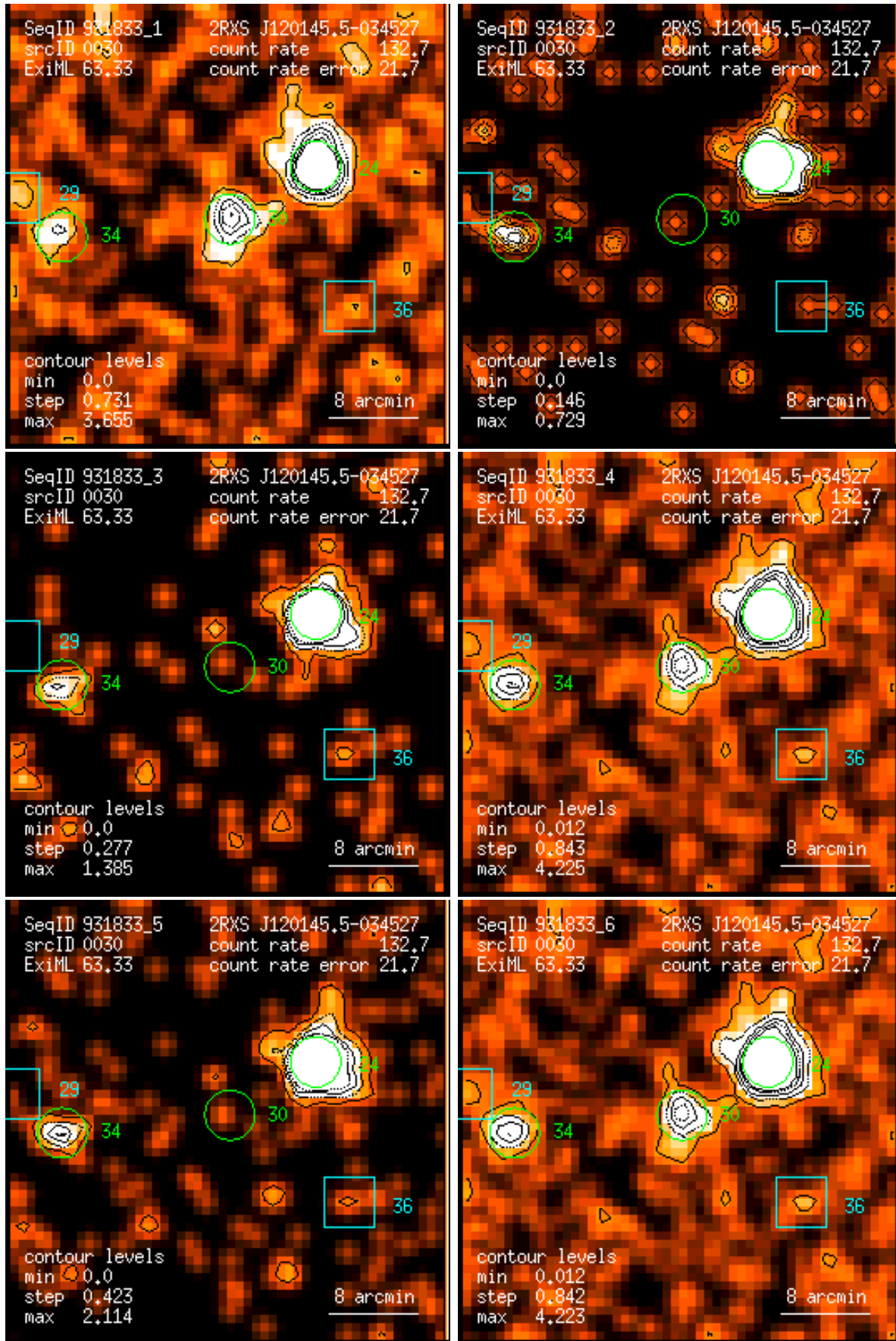
Figure 30: RASS 931833: detection 0030: band rate images, Gaussian filter: (1) PSPC channels 11 – 41, (2) 52 – 90, (3) 91 – 201, (4) 11 – 235, (5) 52 – 201, (6) 11 – 201. Broad band rates in counts/ks. Band rate contour levels in counts/ks/arcmin 2 .
