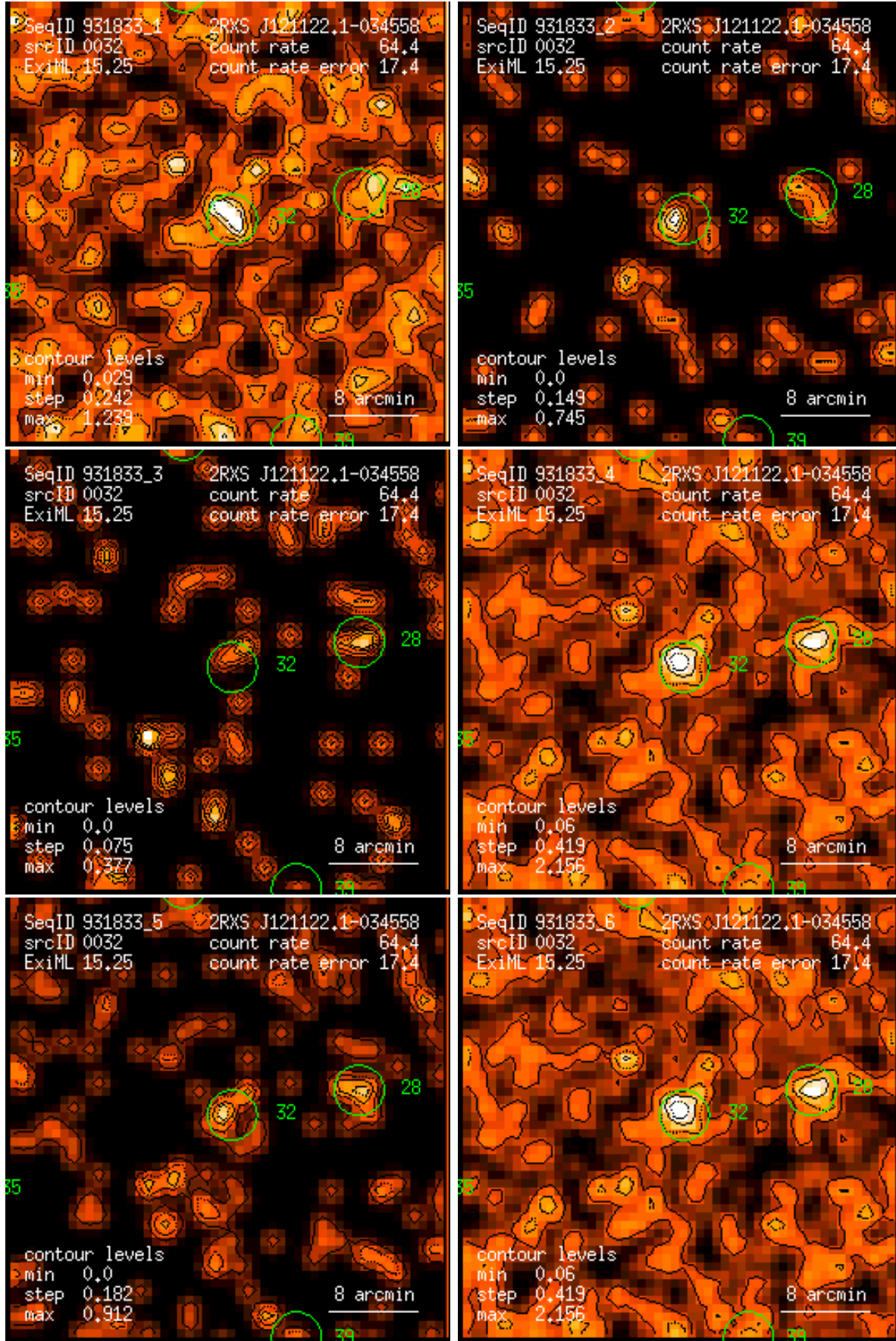
Figure 32: RASS 931833: detection 0032: band rate images, Gaussian filter: (1) PSPC channels 11 – 41, (2) 52 – 90, (3) 91 – 201, (4) 11 – 235, (5) 52 – 201, (6) 11 – 201. Broad band rates in counts/ks. Band rate contour levels in counts/ks/arcmin 2 .
