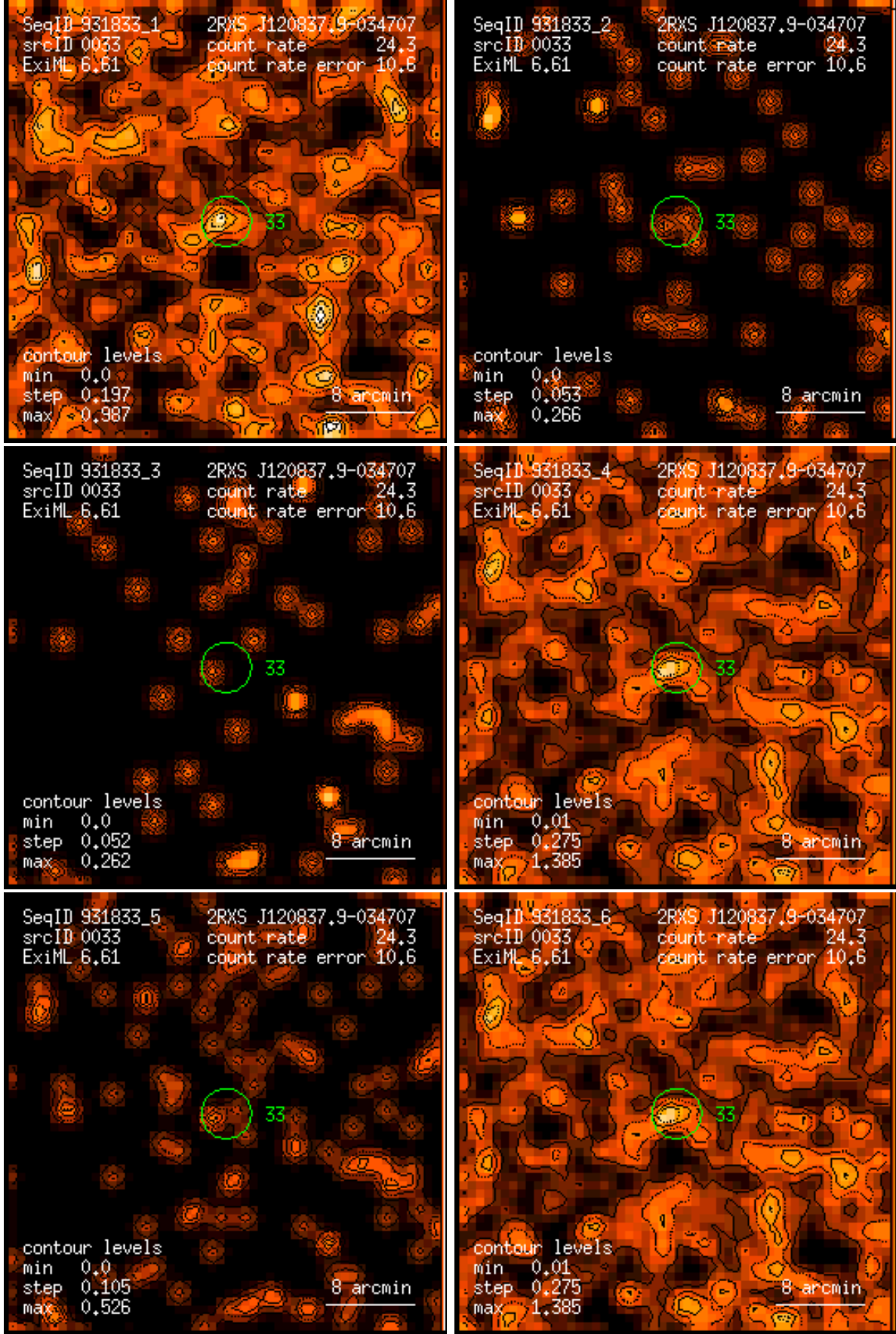
Figure 33: RASS 931833: detection 0033: band rate images, Gaussian filter: (1) PSPC channels 11 – 41, (2) 52 – 90, (3) 91 – 201, (4) 11 – 235, (5) 52 – 201, (6) 11 – 201. Broad band rates in counts/ks. Band rate contour levels in counts/ks/arcmin 2 .
