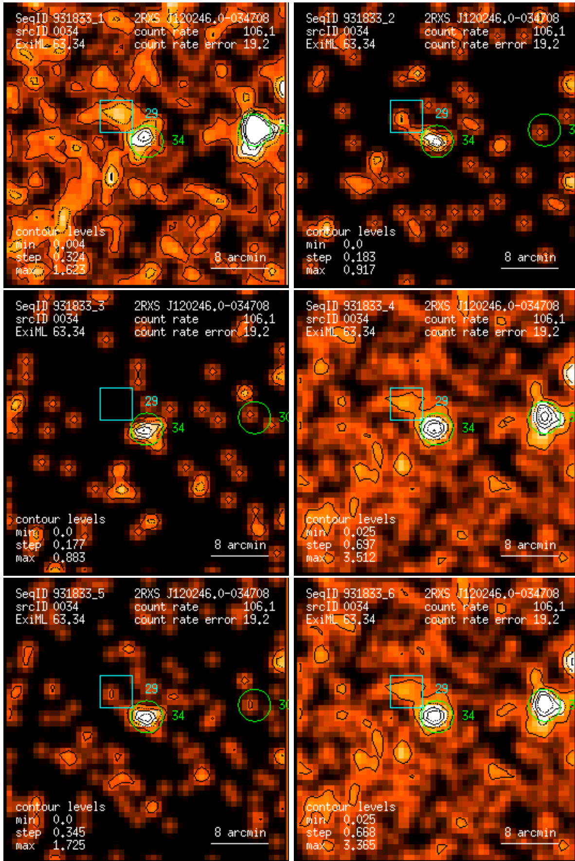
Figure 34: RASS 931833: detection 0034: band rate images, Gaussian filter: (1) PSPC channels 11 – 41, (2) 52 – 90, (3) 91 – 201, (4) 11 – 235, (5) 52 – 201, (6) 11 – 201. Broad band rates in counts/ks. Band rate contour levels in counts/ks/arcmin 2 .
