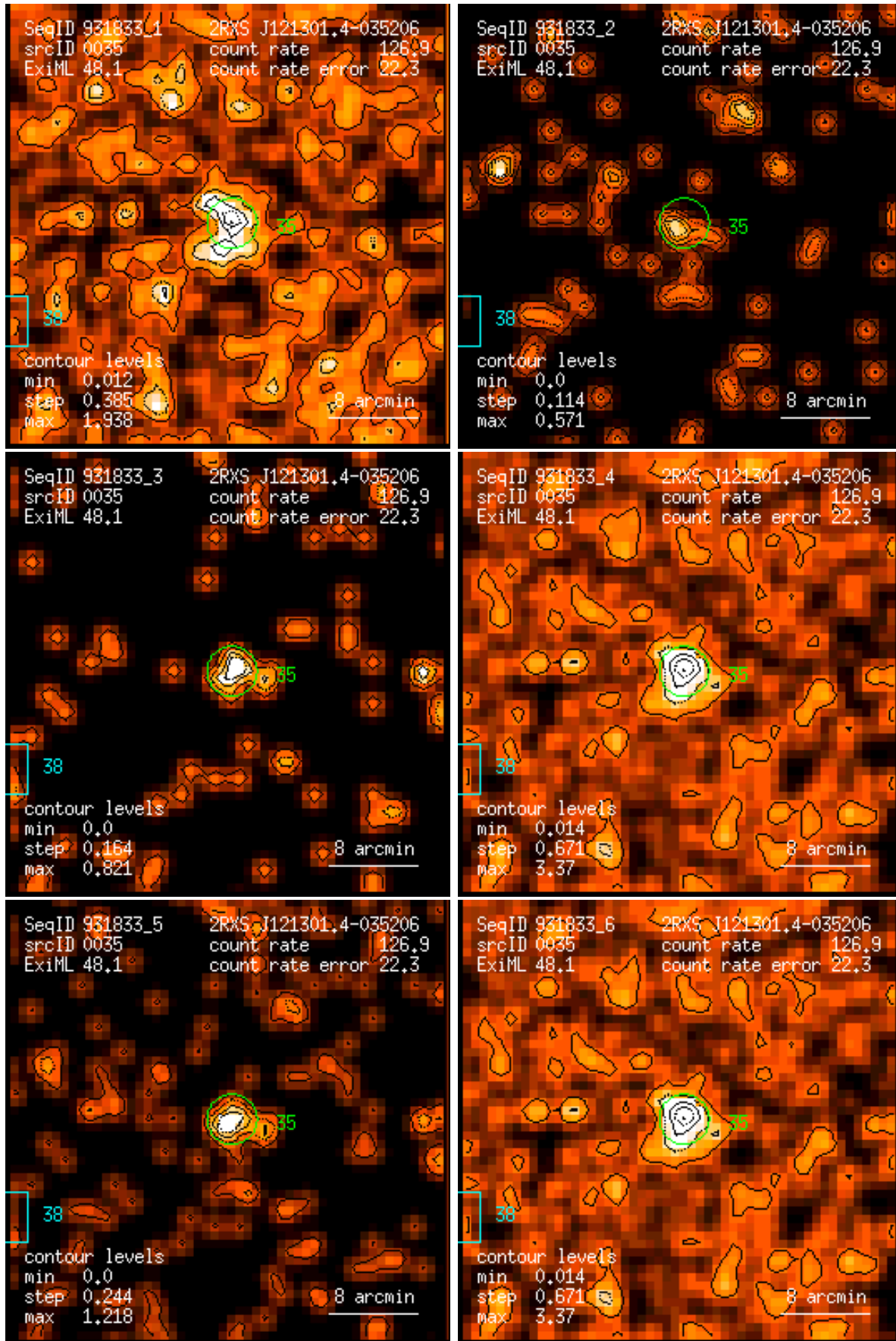
Figure 35: RASS 931833: detection 0035: band rate images, Gaussian filter: (1) PSPC channels 11 – 41, (2) 52 – 90, (3) 91 – 201, (4) 11 – 235, (5) 52 – 201, (6) 11 – 201. Broad band rates in counts/ks. Band rate contour levels in counts/ks/arcmin 2 .
