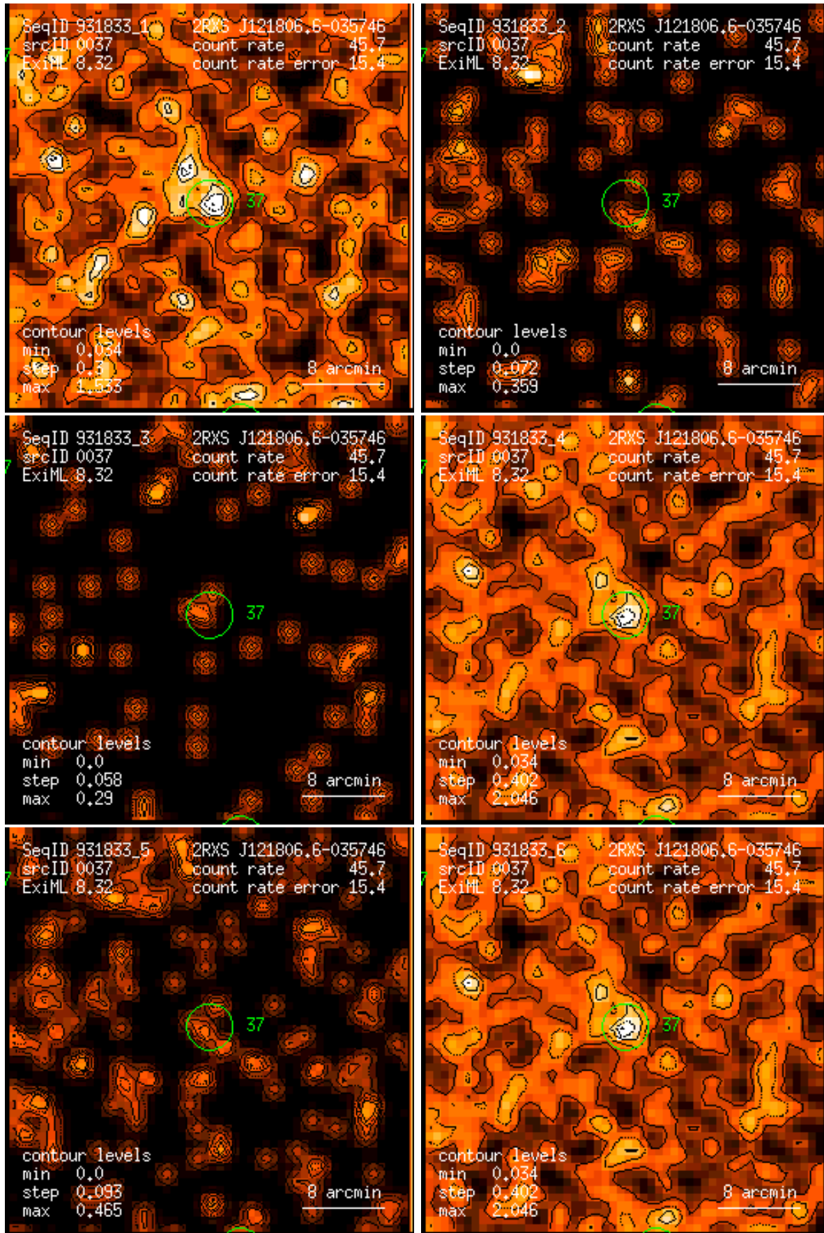
Figure 37: RASS 931833: detection 0037: band rate images, Gaussian filter: (1) PSPC channels 11 – 41, (2) 52 – 90, (3) 91 – 201, (4) 11 – 235, (5) 52 – 201, (6) 11 – 201. Broad band rates in counts/ks. Band rate contour levels in counts/ks/arcmin 2 .
