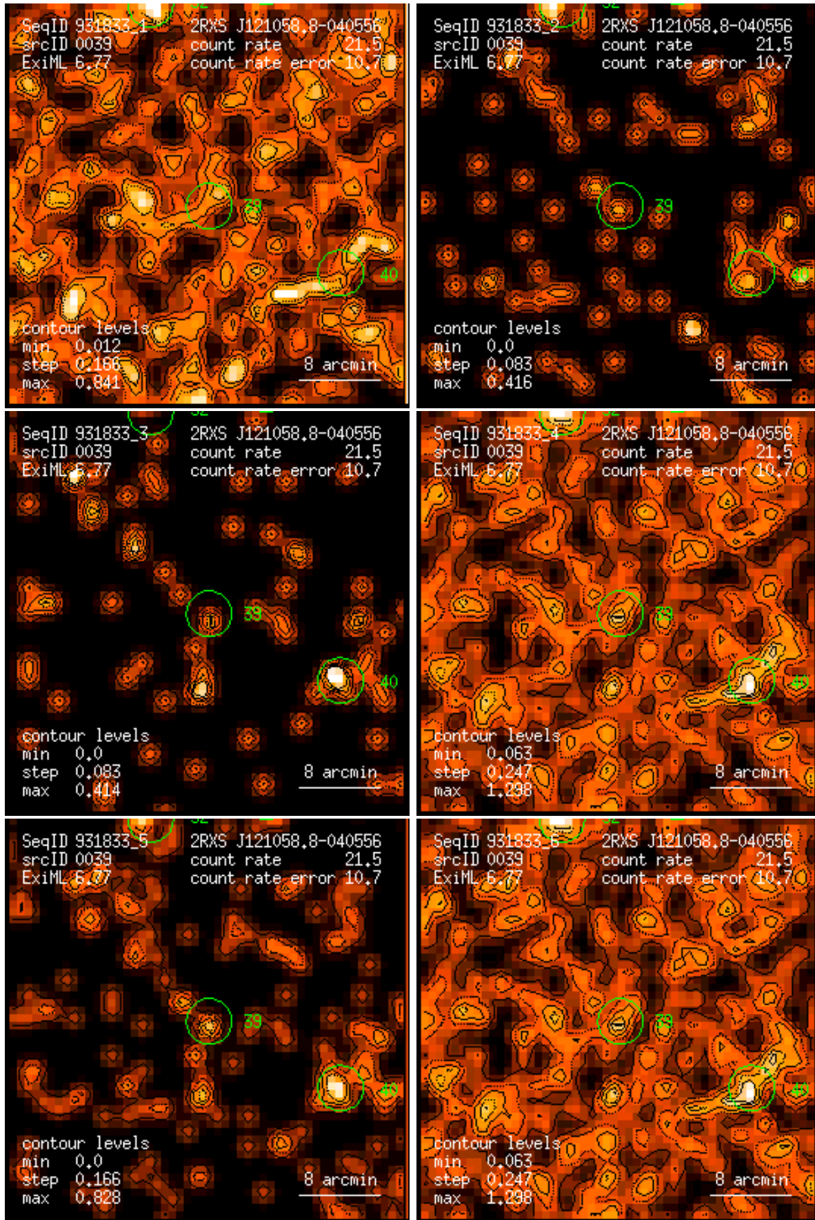
Figure 39: RASS 931833: detection 0039: band rate images, Gaussian filter: (1) PSPC channels 11 – 41, (2) 52 – 90, (3) 91 – 201, (4) 11 – 235, (5) 52 – 201, (6) 11 – 201. Broad band rates in counts/ks. Band rate contour levels in counts/ks/arcmin 2 .
