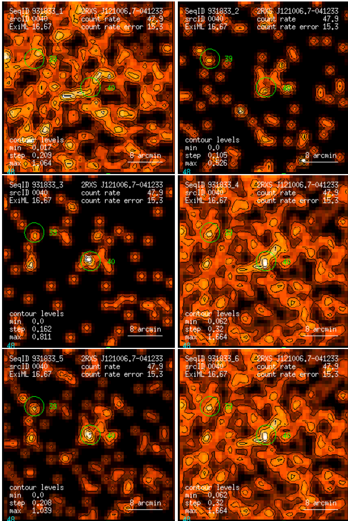
Figure 40: RASS 931833: detection 0040: band rate images, Gaussian filter: (1) PSPC channels 11 – 41, (2) 52 – 90, (3) 91 – 201, (4) 11 – 235, (5) 52 – 201, (6) 11 – 201. Broad band rates in counts/ks. Band rate contour levels in counts/ks/arcmin 2 .
