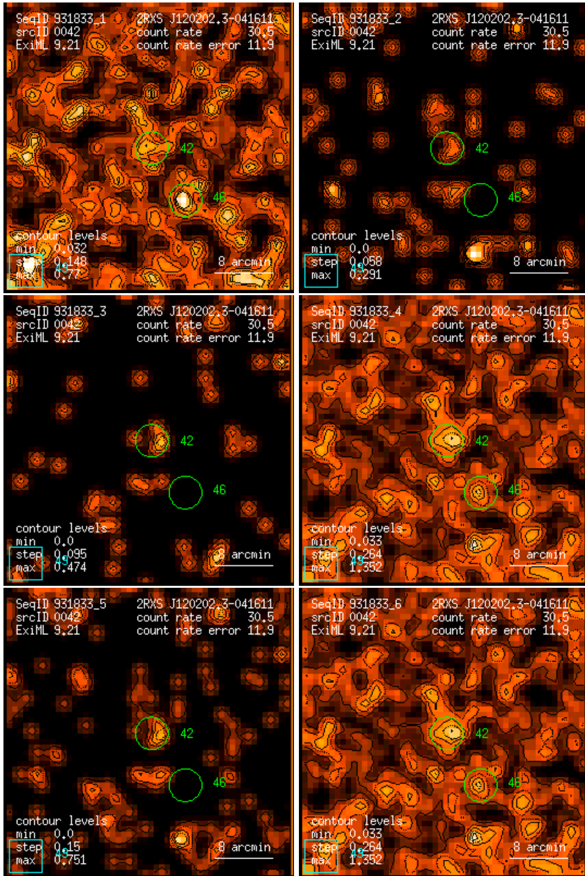
Figure 42: RASS 931833: detection 0042: band rate images, Gaussian filter: (1) PSPC channels 11 – 41, (2) 52 – 90, (3) 91 – 201, (4) 11 – 235, (5) 52 – 201, (6) 11 – 201. Broad band rates in counts/ks. Band rate contour levels in counts/ks/arcmin 2 .
