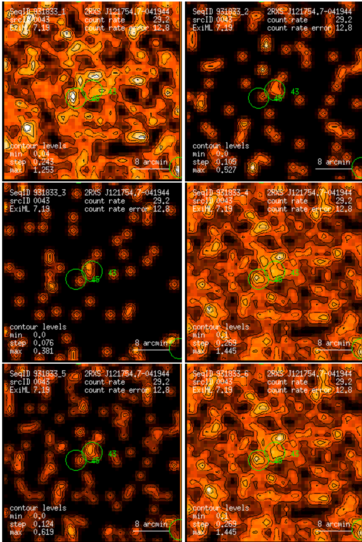
Figure 43: RASS 931833: detection 0043: band rate images, Gaussian filter: (1) PSPC channels 11 – 41, (2) 52 – 90, (3) 91 – 201, (4) 11 – 235, (5) 52 – 201, (6) 11 – 201. Broad band rates in counts/ks. Band rate contour levels in counts/ks/arcmin 2 .
