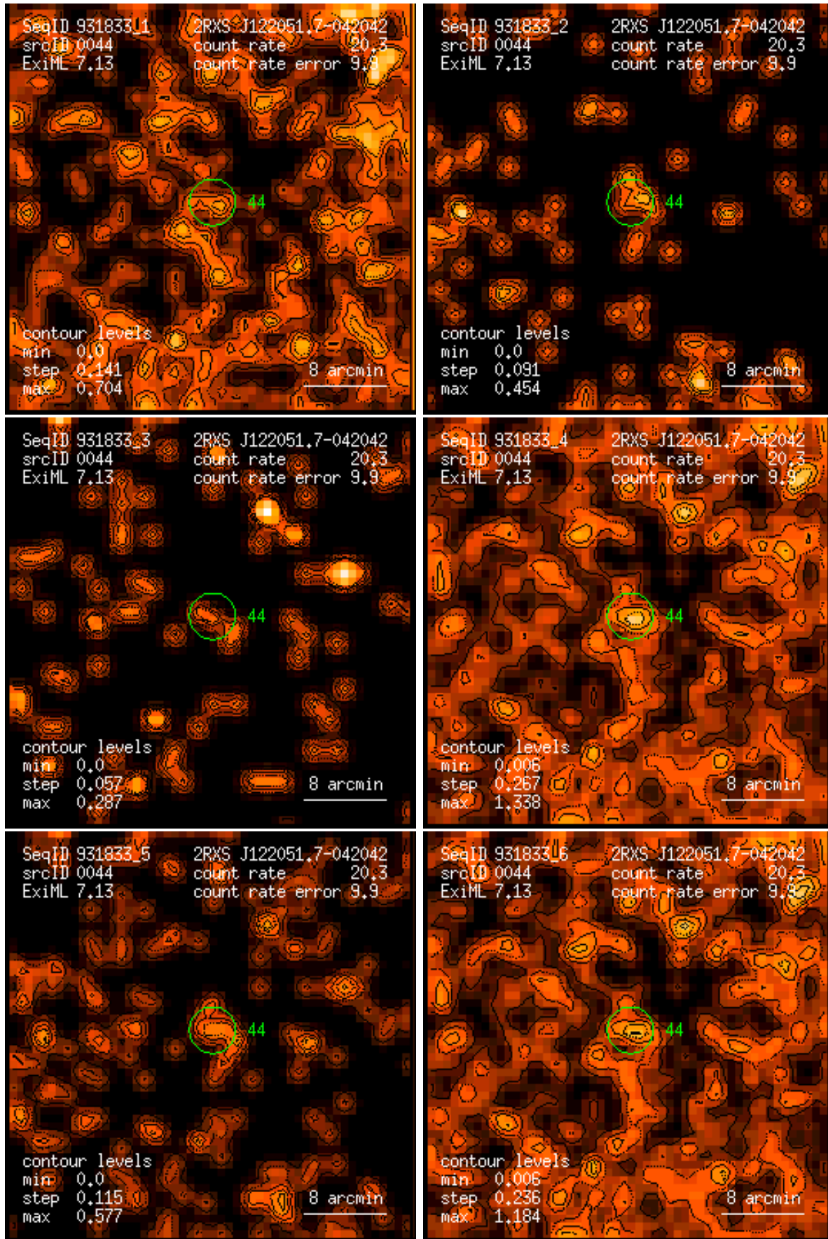
Figure 44: RASS 931833: detection 0044: band rate images, Gaussian filter: (1) PSPC channels 11 – 41, (2) 52 – 90, (3) 91 – 201, (4) 11 – 235, (5) 52 – 201, (6) 11 – 201. Broad band rates in counts/ks. Band rate contour levels in counts/ks/arcmin 2 .
