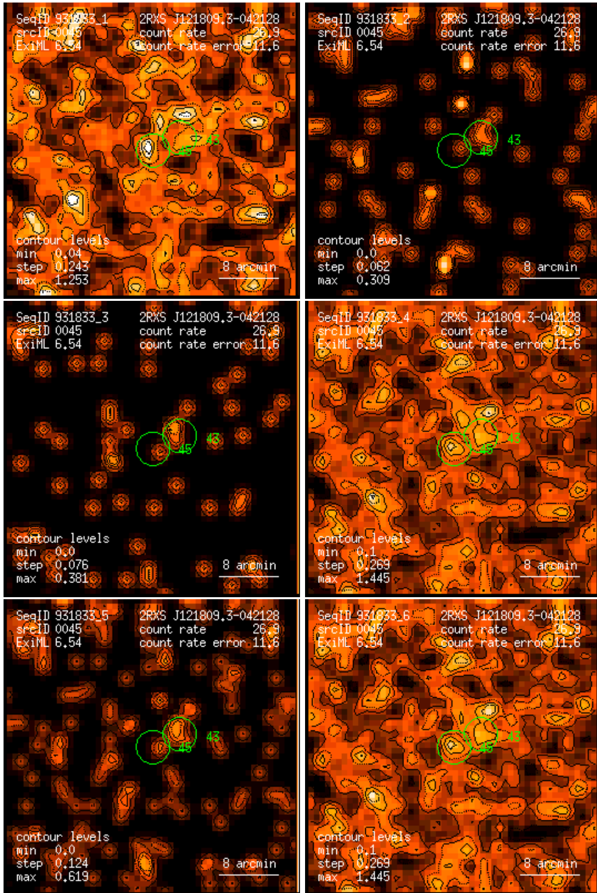
Figure 45: RASS 931833: detection 0045: band rate images, Gaussian filter: (1) PSPC channels 11 – 41, (2) 52 – 90, (3) 91 – 201, (4) 11 – 235, (5) 52 – 201, (6) 11 – 201. Broad band rates in counts/ks. Band rate contour levels in counts/ks/arcmin 2 .
