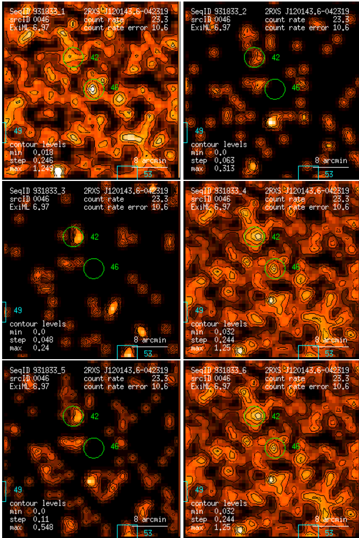
Figure 46: RASS 931833: detection 0046: band rate images, Gaussian filter: (1) PSPC channels 11 – 41, (2) 52 – 90, (3) 91 – 201, (4) 11 – 235, (5) 52 – 201, (6) 11 – 201. Broad band rates in counts/ks. Band rate contour levels in counts/ks/arcmin 2 .
