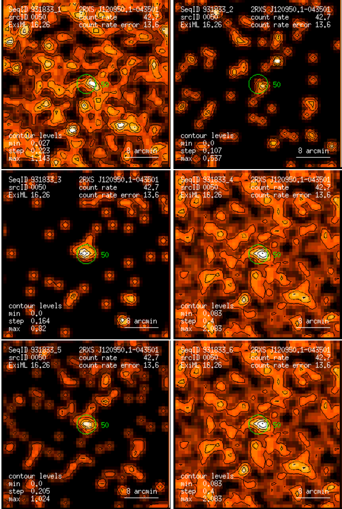
Figure 50: RASS 931833: detection 0050: band rate images, Gaussian filter: (1) PSPC channels 11 – 41, (2) 52 – 90, (3) 91 – 201, (4) 11 – 235, (5) 52 – 201, (6) 11 – 201. Broad band rates in counts/ks. Band rate contour levels in counts/ks/arcmin 2 .
