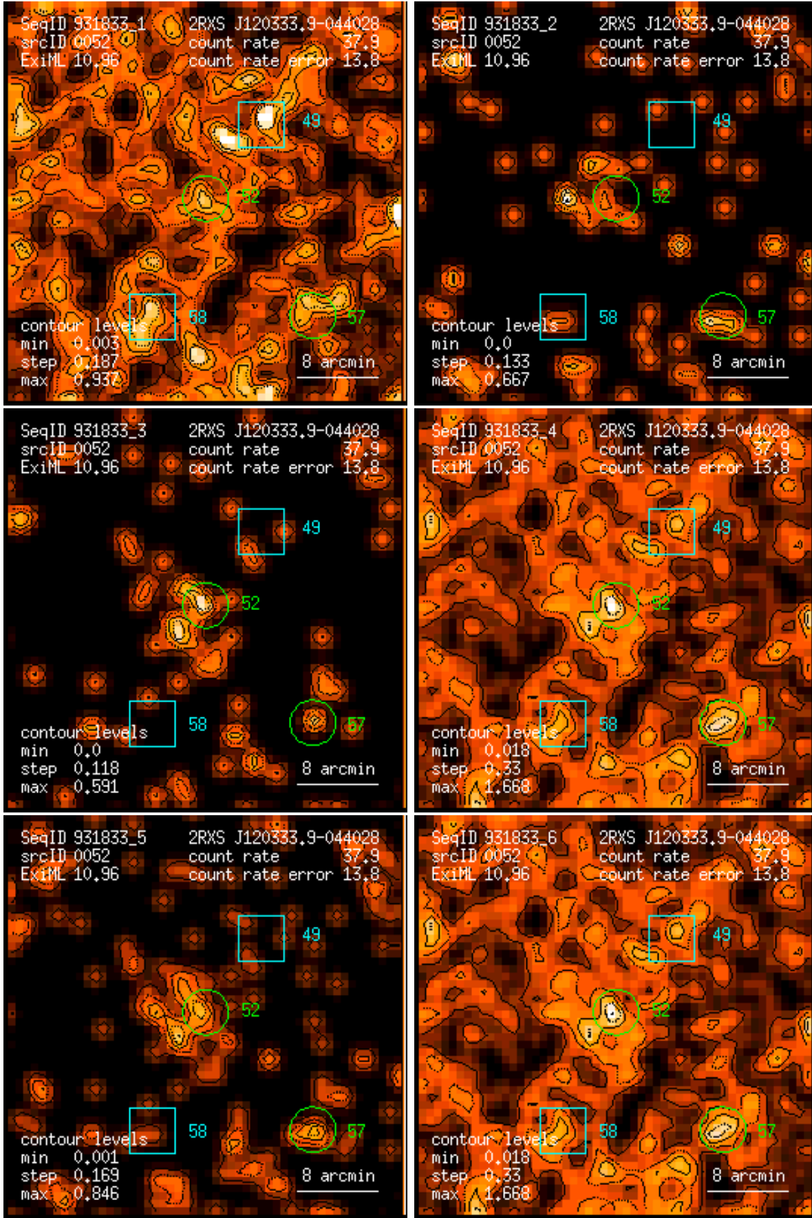
Figure 52: RASS 931833: detection 0052: band rate images, Gaussian filter: (1) PSPC channels 11 – 41, (2) 52 – 90, (3) 91 – 201, (4) 11 – 235, (5) 52 – 201, (6) 11 – 201. Broad band rates in counts/ks. Band rate contour levels in counts/ks/arcmin 2 .
