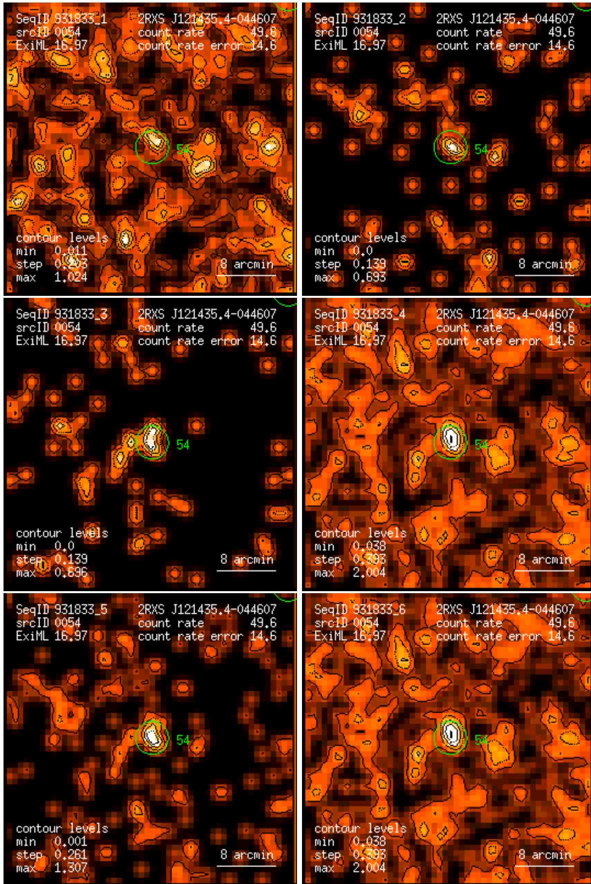
Figure 54: RASS 931833: detection 0054: band rate images, Gaussian filter: (1) PSPC channels 11 – 41, (2) 52 – 90, (3) 91 – 201, (4) 11 – 235, (5) 52 – 201, (6) 11 – 201. Broad band rates in counts/ks. Band rate contour levels in counts/ks/arcmin 2 .
