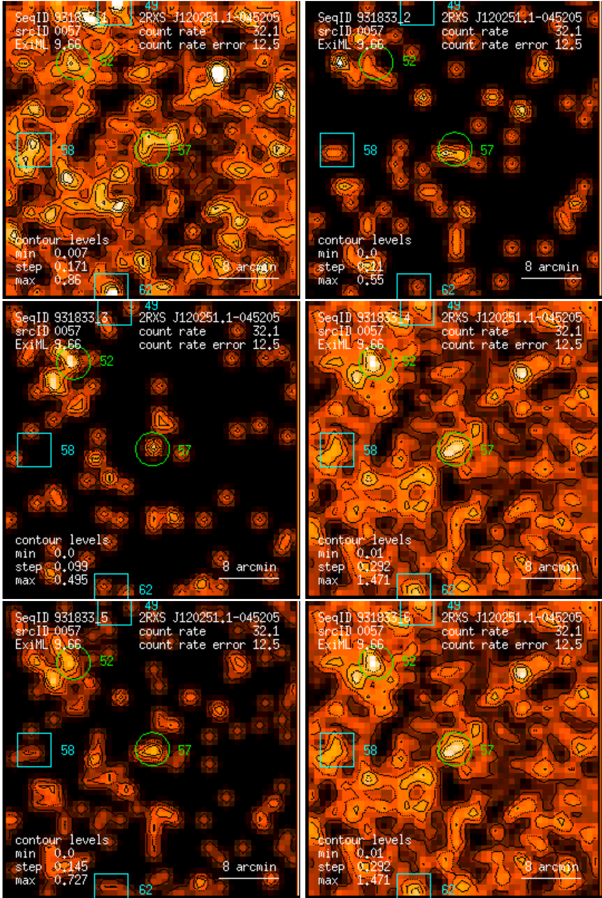
Figure 57: RASS 931833: detection 0057: band rate images, Gaussian filter: (1) PSPC channels 11 – 41, (2) 52 – 90, (3) 91 – 201, (4) 11 – 235, (5) 52 – 201, (6) 11 – 201. Broad band rates in counts/ks. Band rate contour levels in counts/ks/arcmin 2 .
