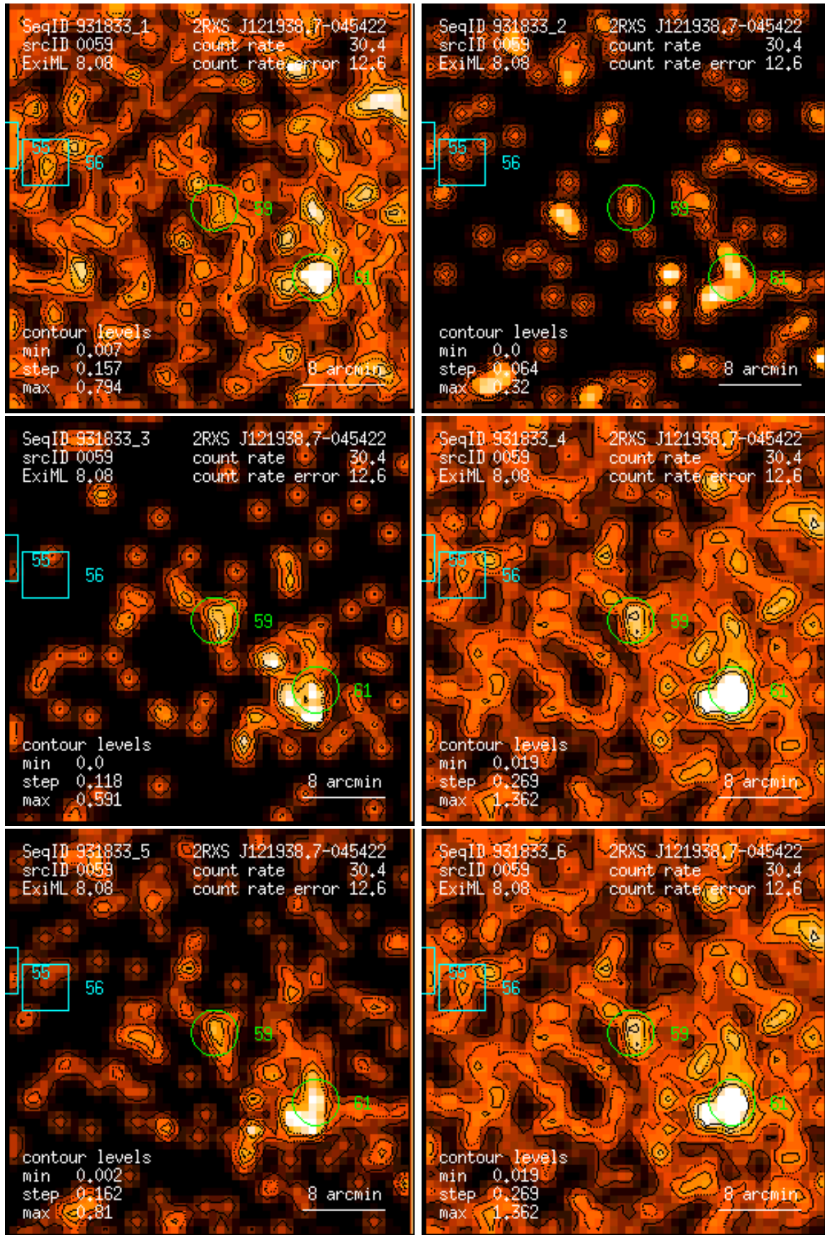
Figure 59: RASS 931833: detection 0059: band rate images, Gaussian filter: (1) PSPC channels 11 – 41, (2) 52 – 90, (3) 91 – 201, (4) 11 – 235, (5) 52 – 201, (6) 11 – 201. Broad band rates in counts/ks. Band rate contour levels in counts/ks/arcmin 2 .
