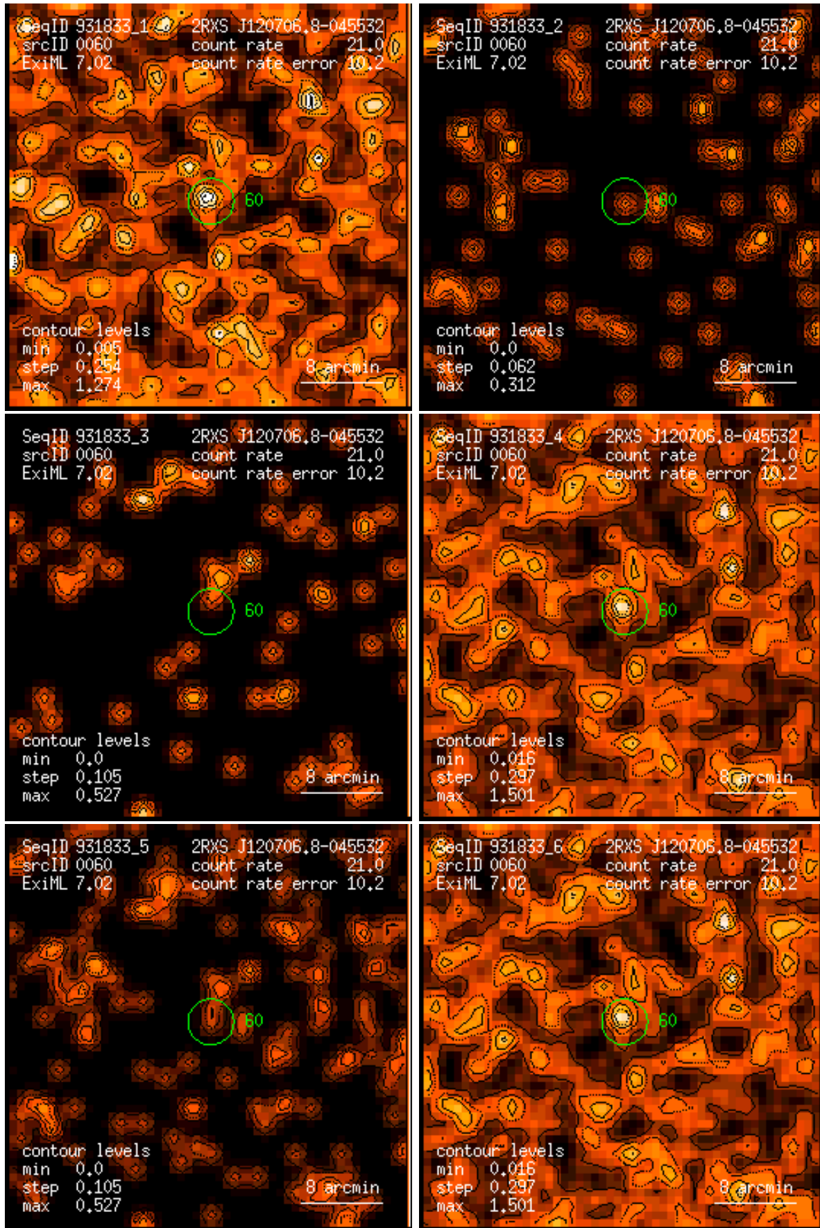
Figure 60: RASS 931833: detection 0060: band rate images, Gaussian filter: (1) PSPC channels 11 – 41, (2) 52 – 90, (3) 91 – 201, (4) 11 – 235, (5) 52 – 201, (6) 11 – 201. Broad band rates in counts/ks. Band rate contour levels in counts/ks/arcmin 2 .
