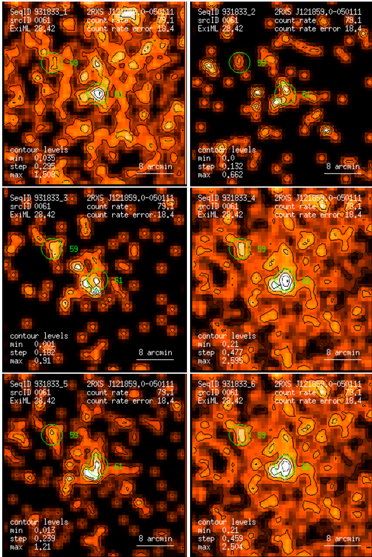
Figure 61: RASS 931833: detection 0061: band rate images, Gaussian filter: (1) PSPC channels 11 – 41, (2) 52 – 90, (3) 91 – 201, (4) 11 – 235, (5) 52 – 201, (6) 11 – 201. Broad band rates in counts/ks. Band rate contour levels in counts/ks/arcmin 2 .
