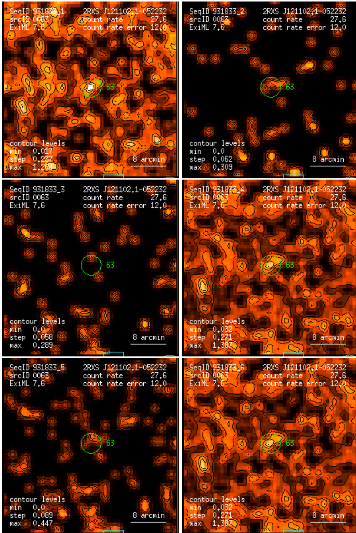
Figure 63: RASS 931833: detection 0063: band rate images, Gaussian filter: (1) PSPC channels 11 – 41, (2) 52 – 90, (3) 91 – 201, (4) 11 – 235, (5) 52 – 201, (6) 11 – 201. Broad band rates in counts/ks. Band rate contour levels in counts/ks/arcmin 2 .
