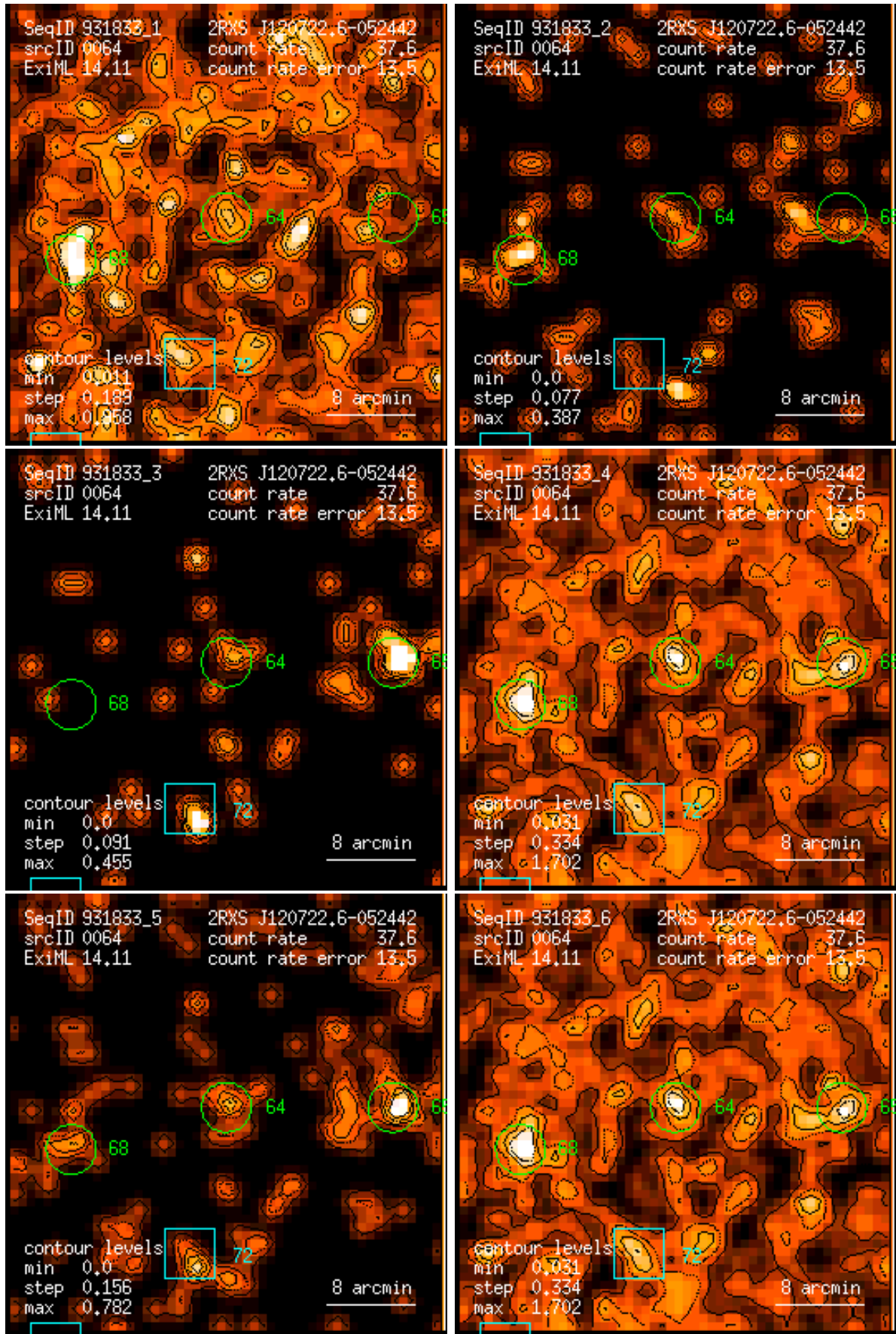
Figure 64: RASS 931833: detection 0064: band rate images, Gaussian filter: (1) PSPC channels 11 – 41, (2) 52 – 90, (3) 91 – 201, (4) 11 – 235, (5) 52 – 201, (6) 11 – 201. Broad band rates in counts/ks. Band rate contour levels in counts/ks/arcmin 2 .
