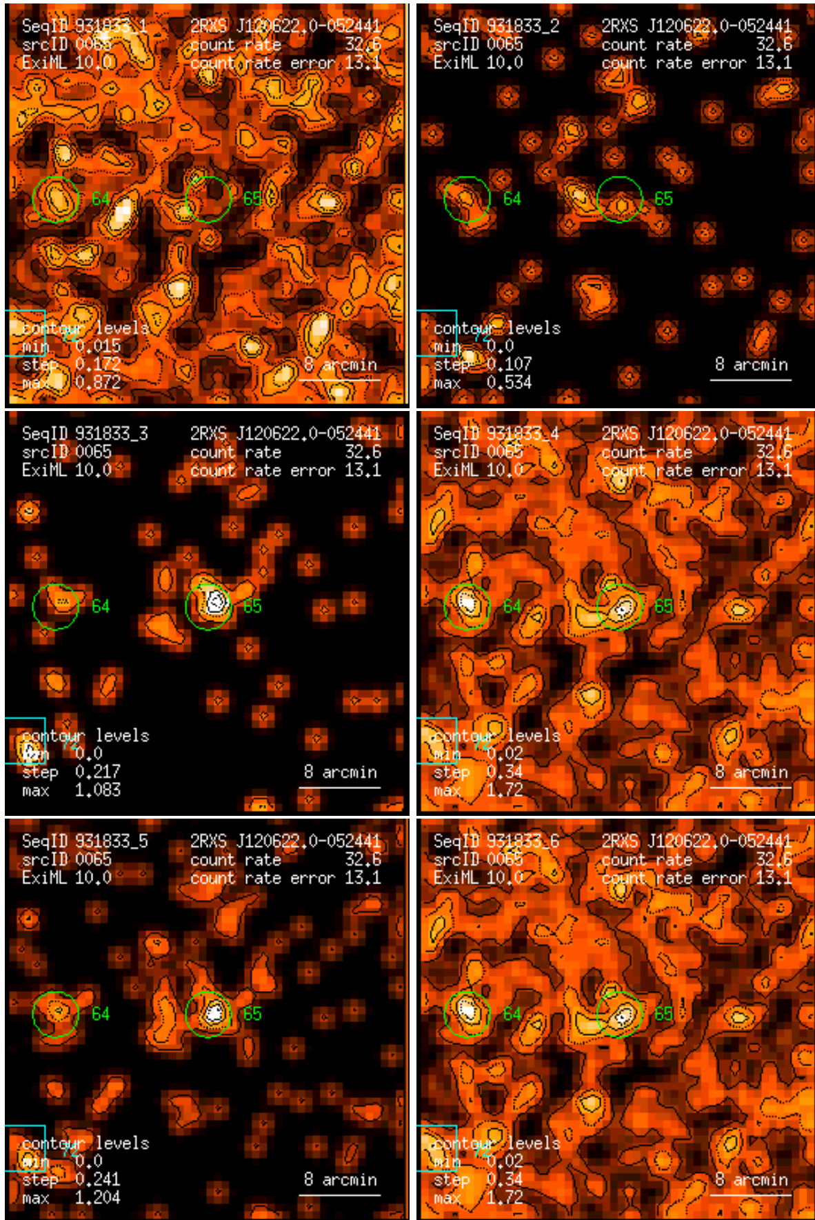
Figure 65: RASS 931833: detection 0065: band rate images, Gaussian filter: (1) PSPC channels 11 – 41, (2) 52 – 90, (3) 91 – 201, (4) 11 – 235, (5) 52 – 201, (6) 11 – 201. Broad band rates in counts/ks. Band rate contour levels in counts/ks/arcmin 2 .
