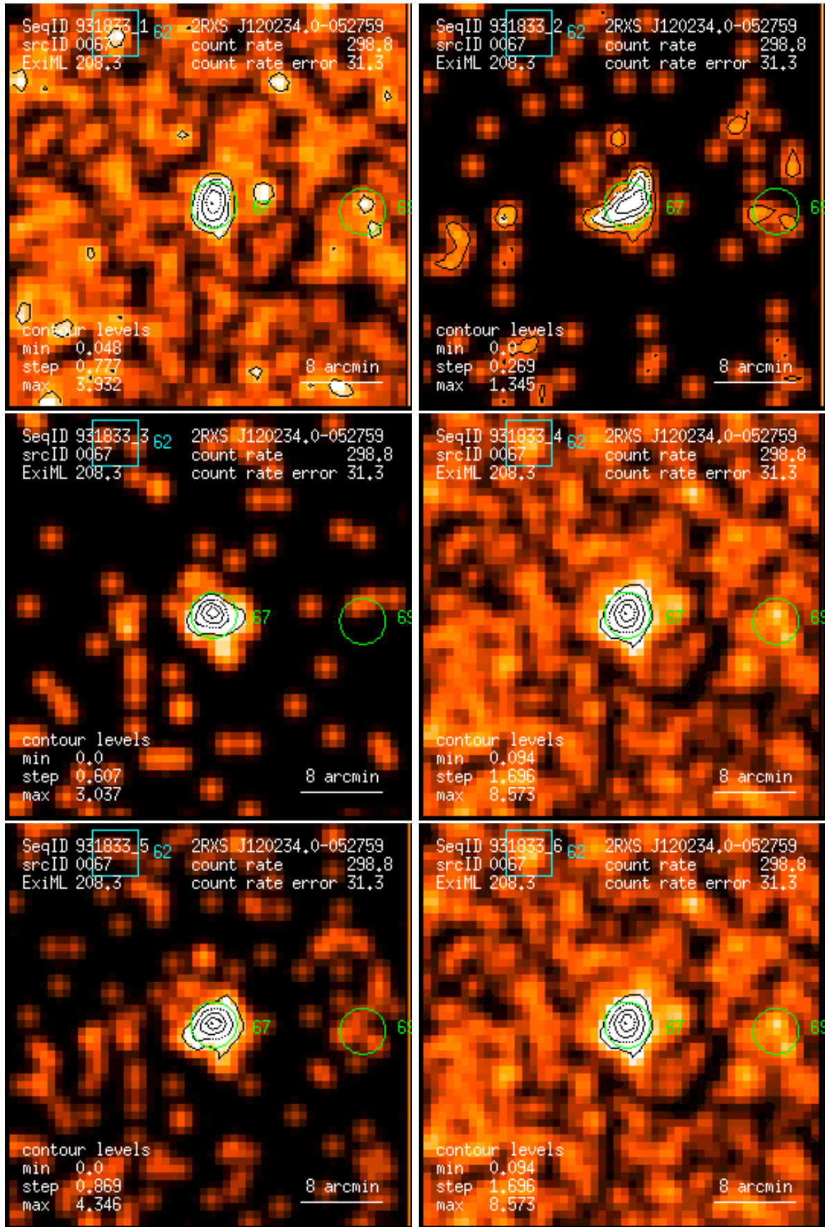
Figure 67: RASS 931833: detection 0067: band rate images, Gaussian filter: (1) PSPC channels 11 – 41, (2) 52 – 90, (3) 91 – 201, (4) 11 – 235, (5) 52 – 201, (6) 11 – 201. Broad band rates in counts/ks. Band rate contour levels in counts/ks/arcmin 2 .
