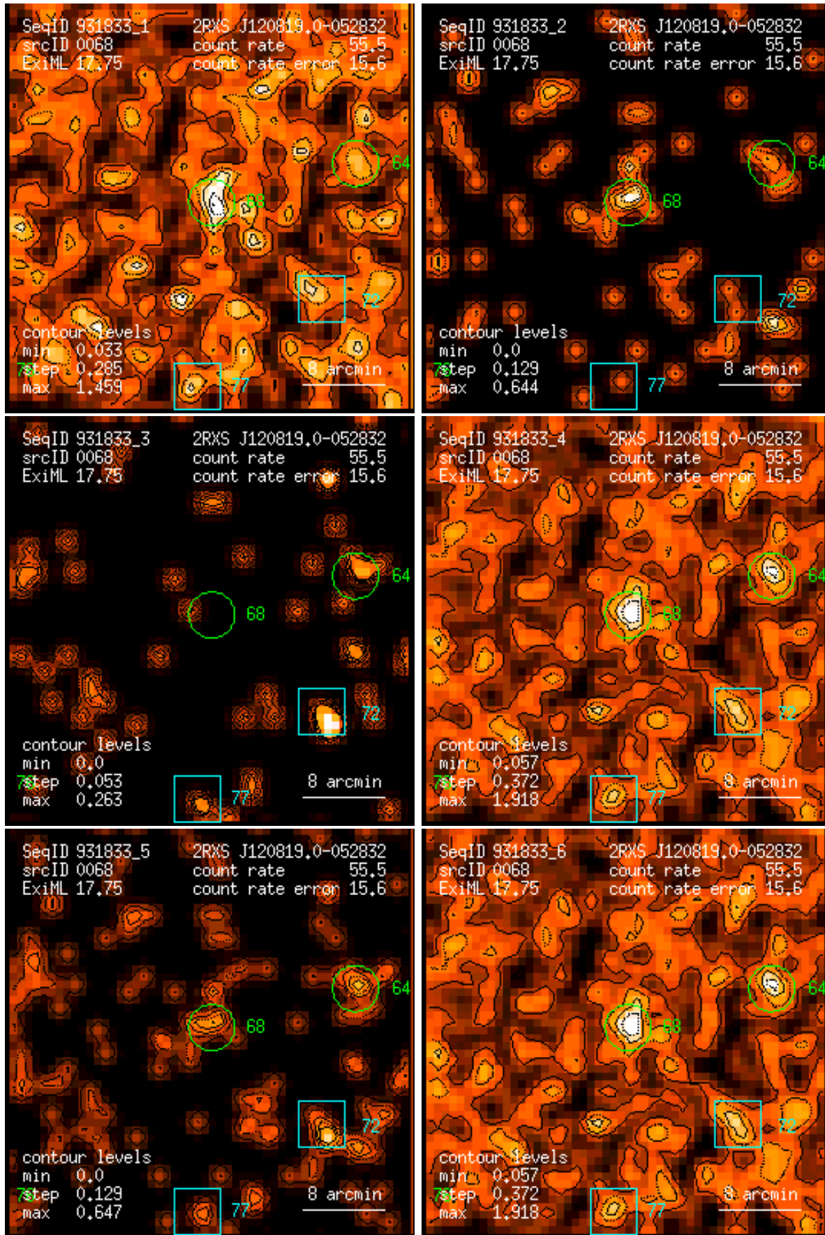
Figure 68: RASS 931833: detection 0068: band rate images, Gaussian filter: (1) PSPC channels 11 – 41, (2) 52 – 90, (3) 91 – 201, (4) 11 – 235, (5) 52 – 201, (6) 11 – 201. Broad band rates in counts/ks. Band rate contour levels in counts/ks/arcmin 2 .
