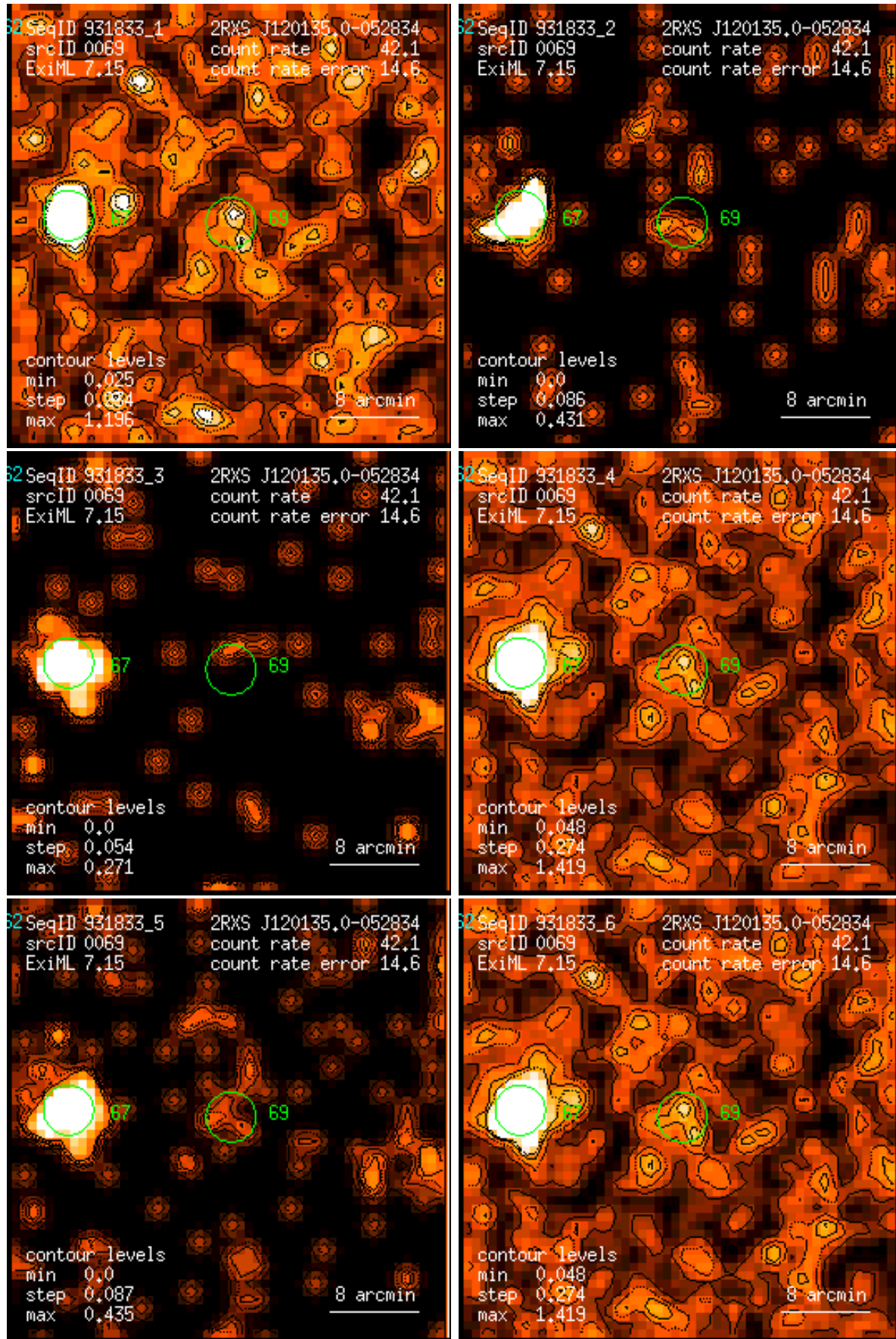
Figure 69: RASS 931833: detection 0069: band rate images, Gaussian filter: (1) PSPC channels 11 – 41, (2) 52 – 90, (3) 91 – 201, (4) 11 – 235, (5) 52 – 201, (6) 11 – 201. Broad band rates in counts/ks. Band rate contour levels in counts/ks/arcmin 2 .
