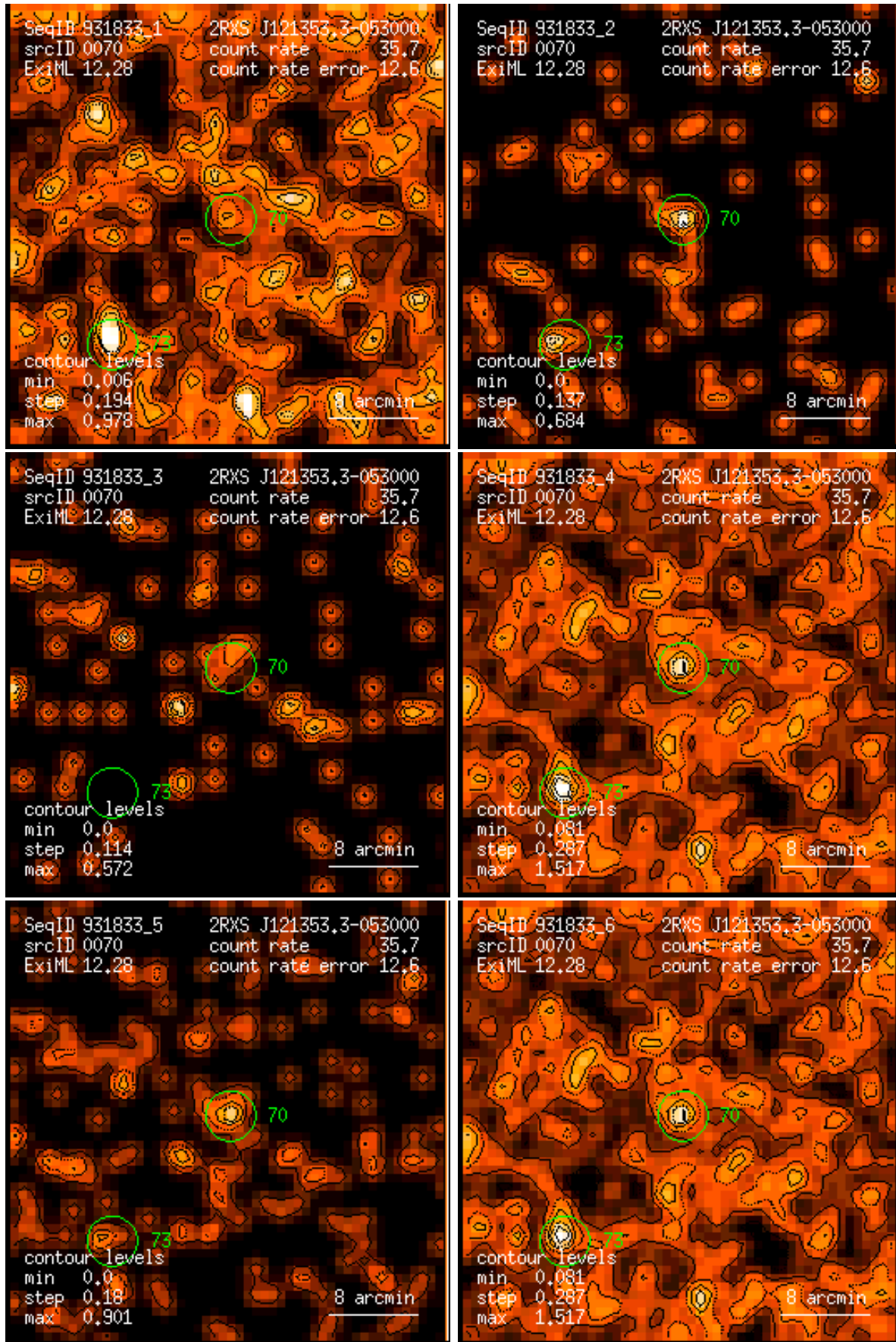
Figure 70: RASS 931833: detection 0070: band rate images, Gaussian filter: (1) PSPC channels 11 – 41, (2) 52 – 90, (3) 91 – 201, (4) 11 – 235, (5) 52 – 201, (6) 11 – 201. Broad band rates in counts/ks. Band rate contour levels in counts/ks/arcmin 2 .
