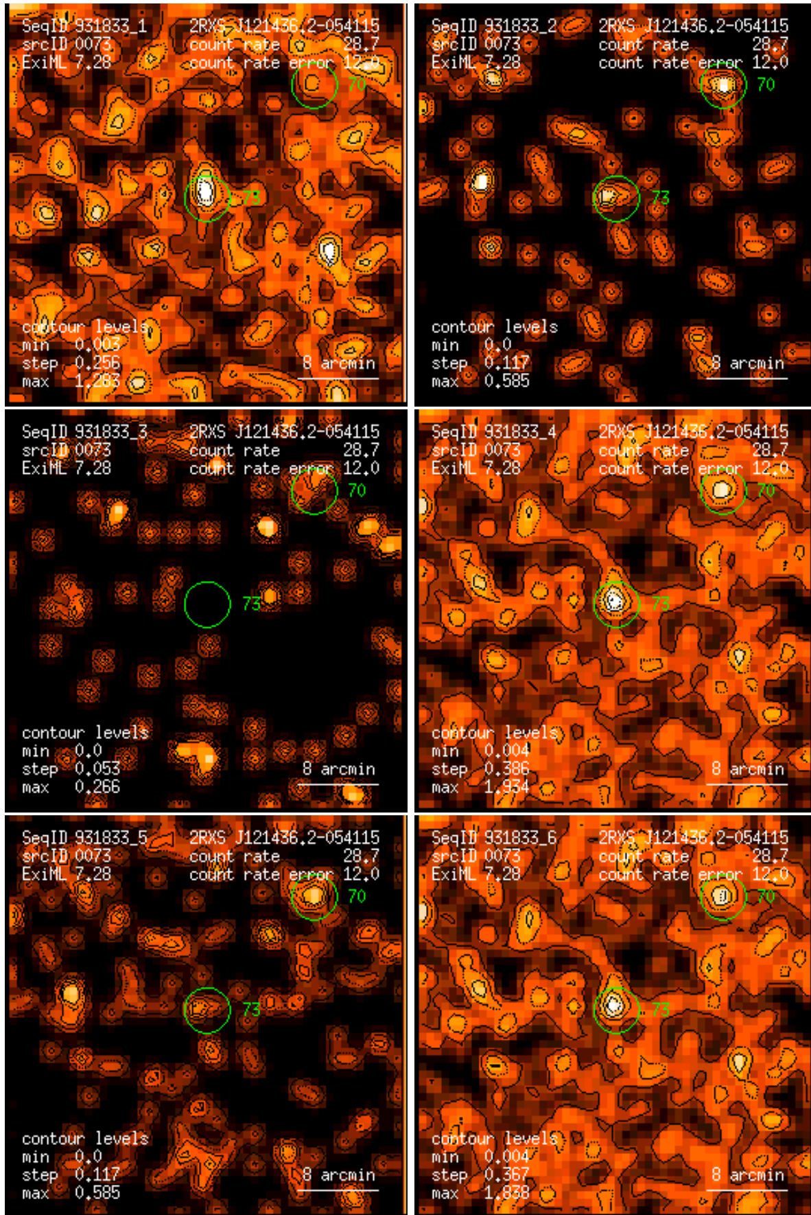
Figure 73: RASS 931833: detection 0073: band rate images, Gaussian filter: (1) PSPC channels 11 – 41, (2) 52 – 90, (3) 91 – 201, (4) 11 – 235, (5) 52 – 201, (6) 11 – 201. Broad band rates in counts/ks. Band rate contour levels in counts/ks/arcmin 2 .
