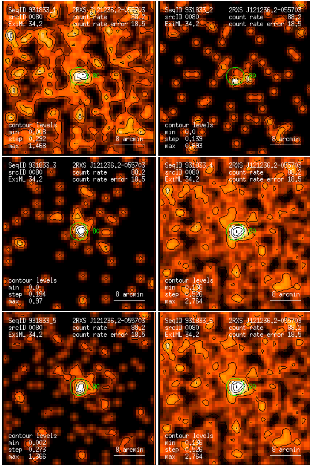
Figure 80: RASS 931833: detection 0080: band rate images, Gaussian filter: (1) PSPC channels 11 – 41, (2) 52 – 90, (3) 91 – 201, (4) 11 – 235, (5) 52 – 201, (6) 11 – 201. Broad band rates in counts/ks. Band rate contour levels in counts/ks/arcmin 2 .
