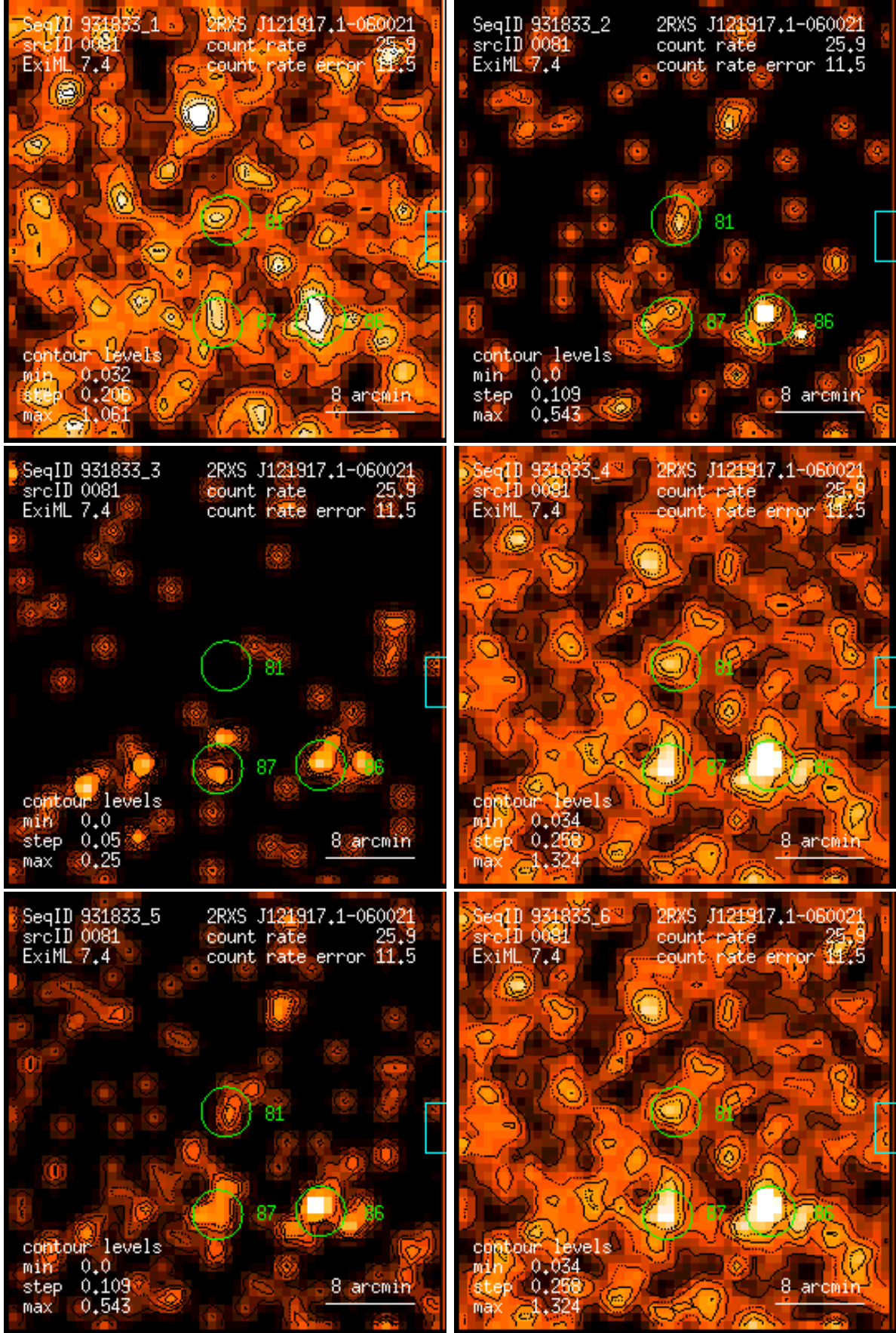
Figure 81: RASS 931833: detection 0081: band rate images, Gaussian filter: (1) PSPC channels 11 – 41, (2) 52 – 90, (3) 91 – 201, (4) 11 – 235, (5) 52 – 201, (6) 11 – 201. Broad band rates in counts/ks. Band rate contour levels in counts/ks/arcmin 2 .
