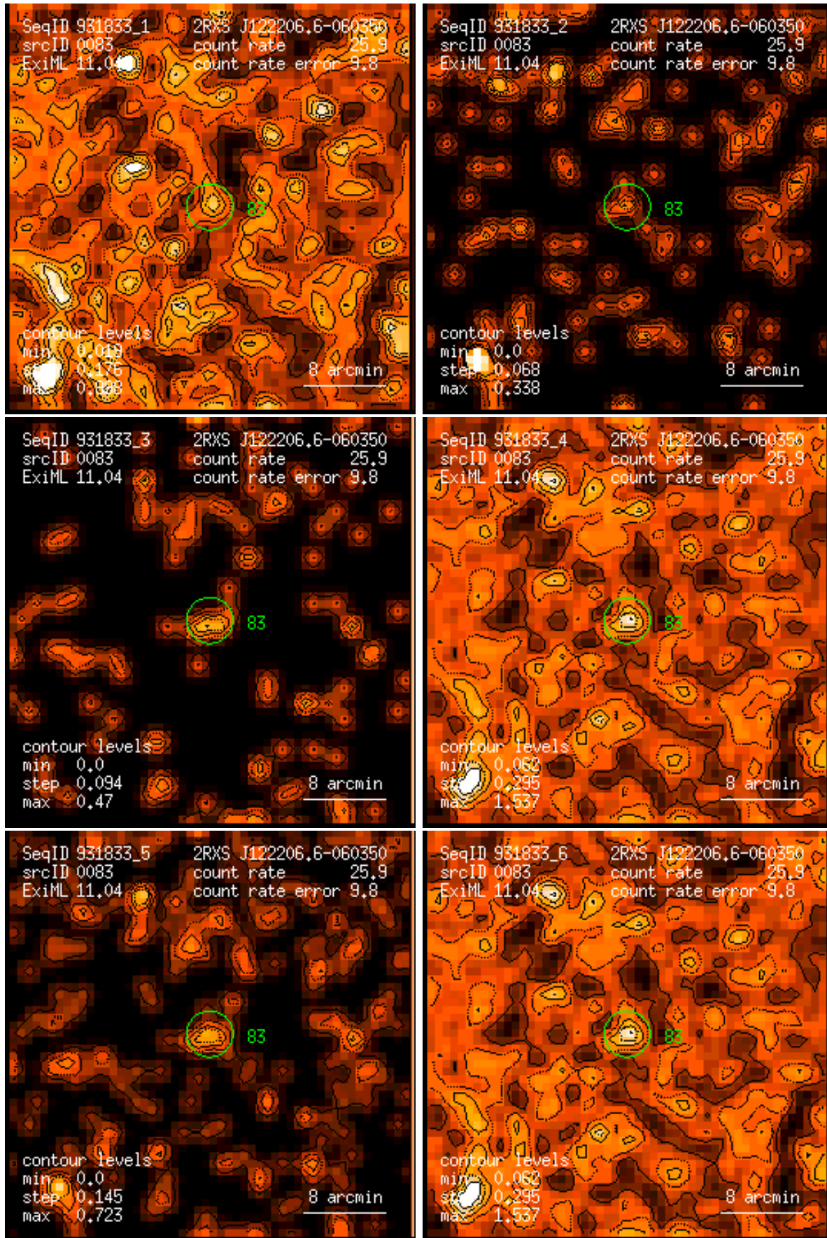
Figure 83: RASS 931833: detection 0083: band rate images, Gaussian filter: (1) PSPC channels 11 – 41, (2) 52 – 90, (3) 91 – 201, (4) 11 – 235, (5) 52 – 201, (6) 11 – 201. Broad band rates in counts/ks. Band rate contour levels in counts/ks/arcmin 2 .
